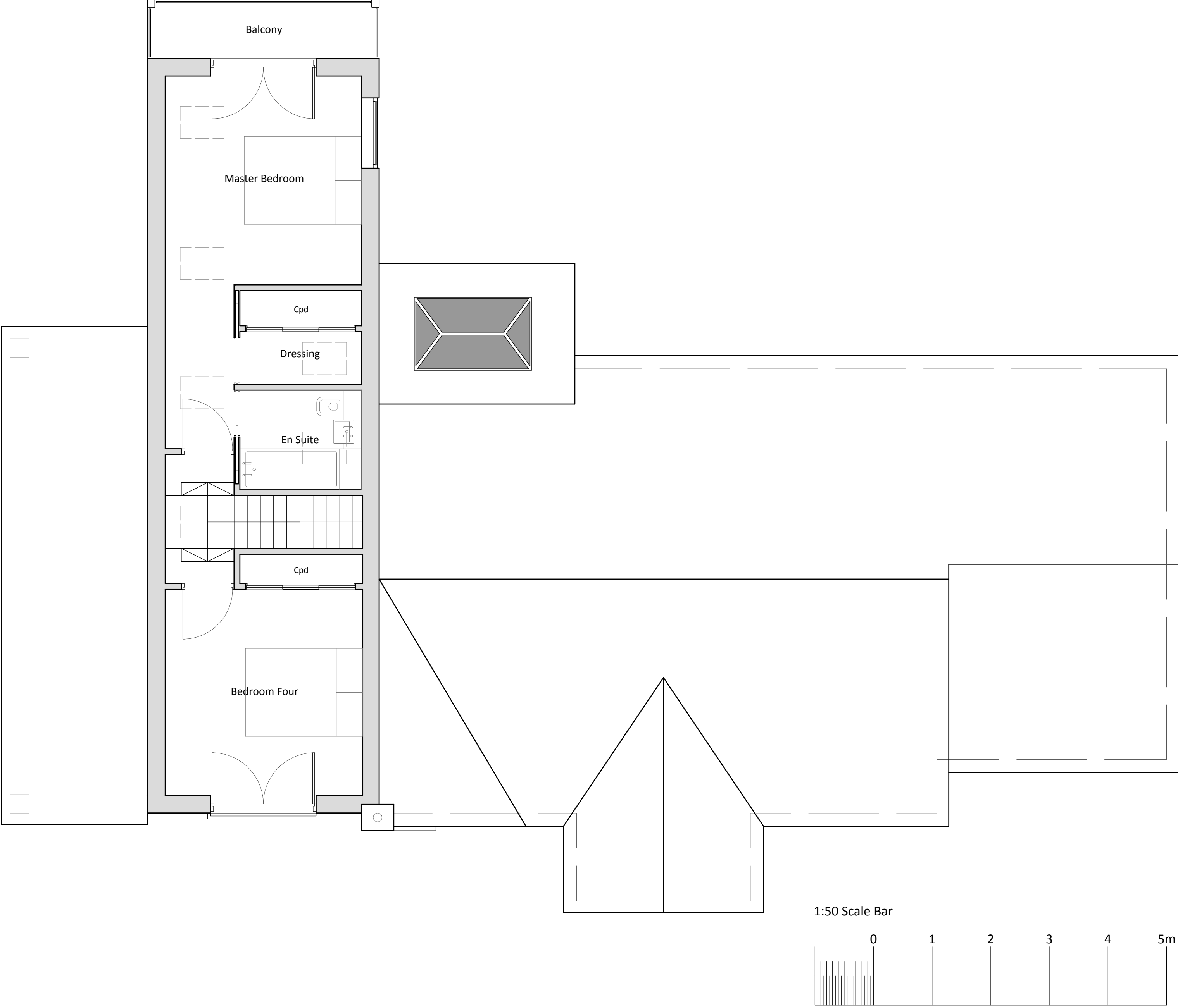
Proposed First Floor Plan 1:50
