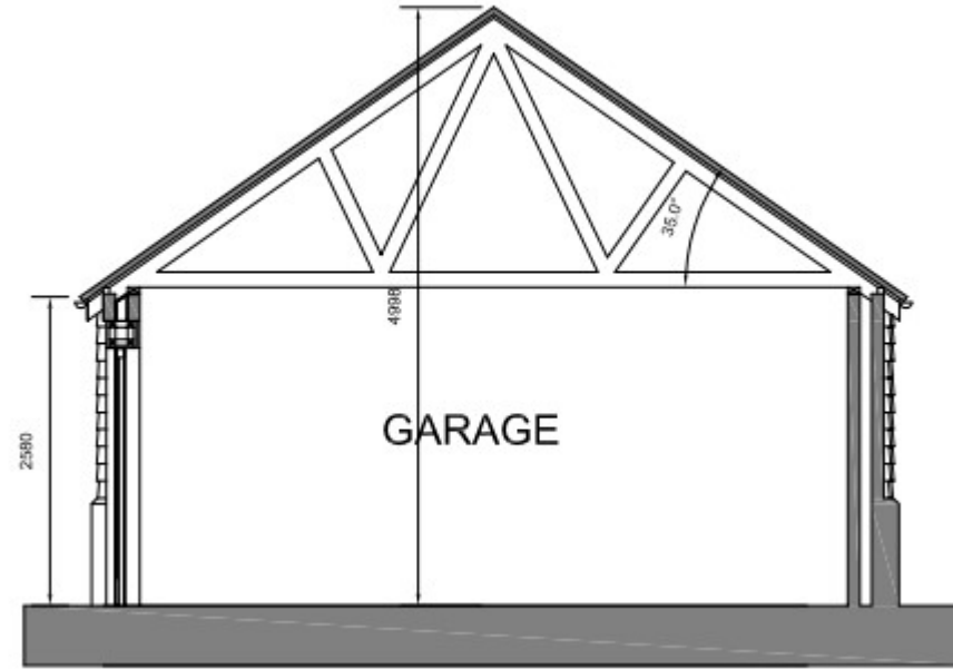
CROSS SECTION
