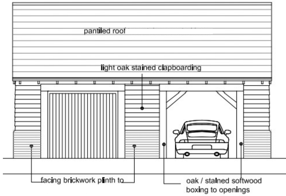
SOUTH ELEVATION
