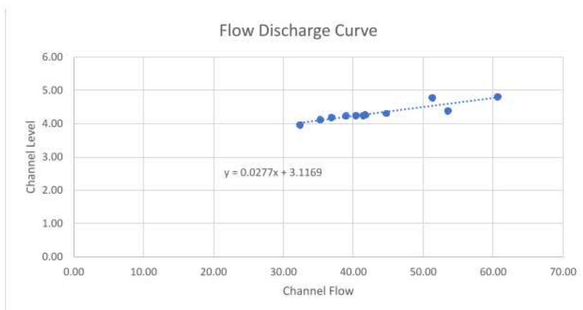
Figure 4 – Flow discharge curve
