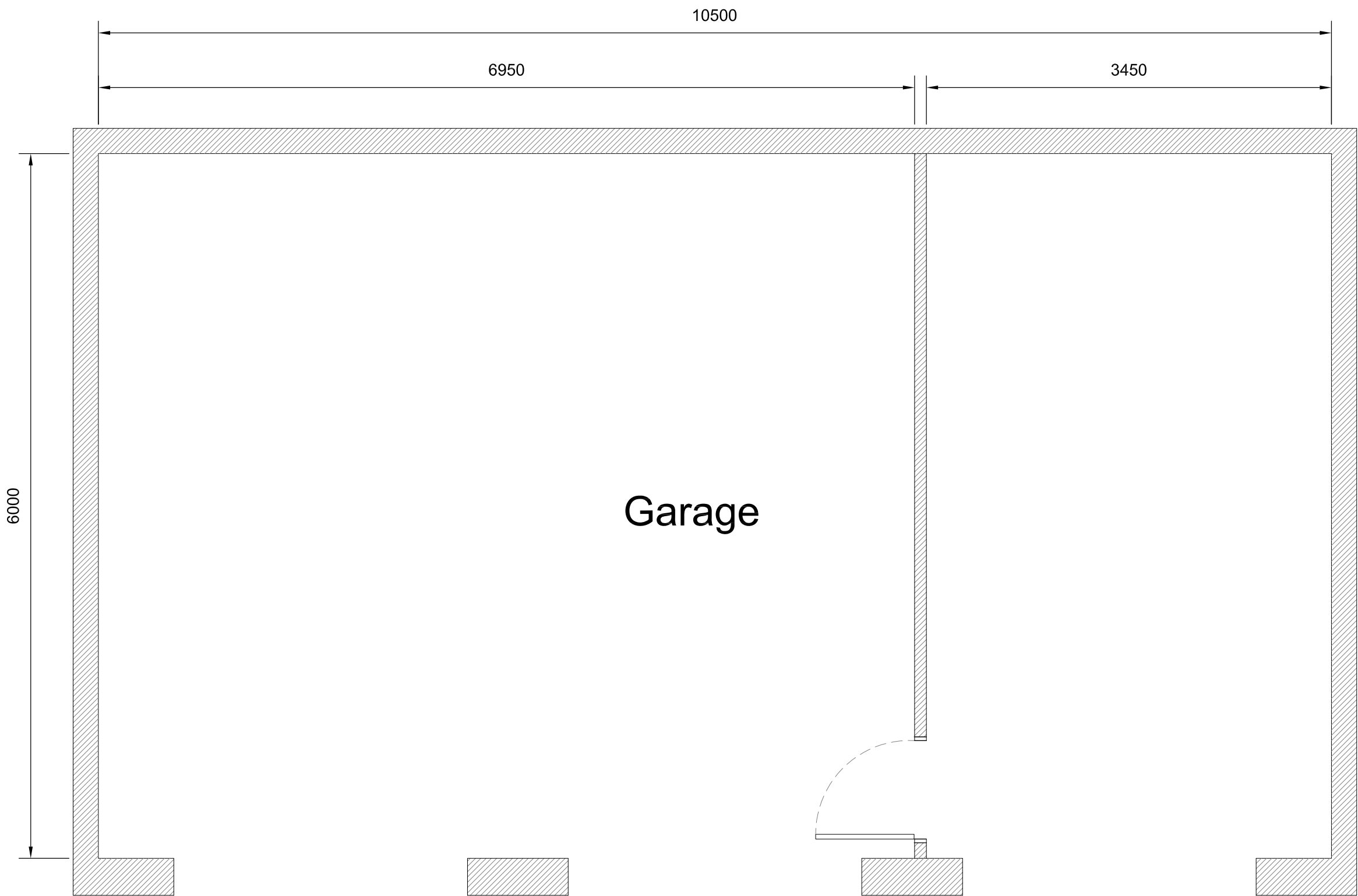
PROPOSED GARAGE FLOOR PLAN
