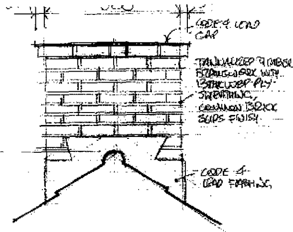
FRONT ELEVATION ON ALL CHIMNEYS EXCEPT AT GABLE ENDS
