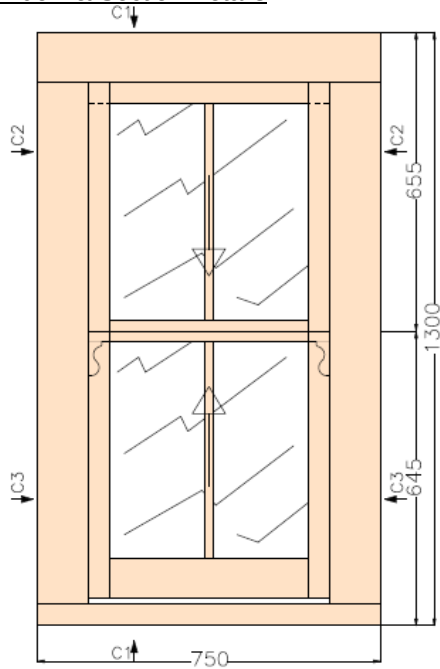
Typical Elevation
