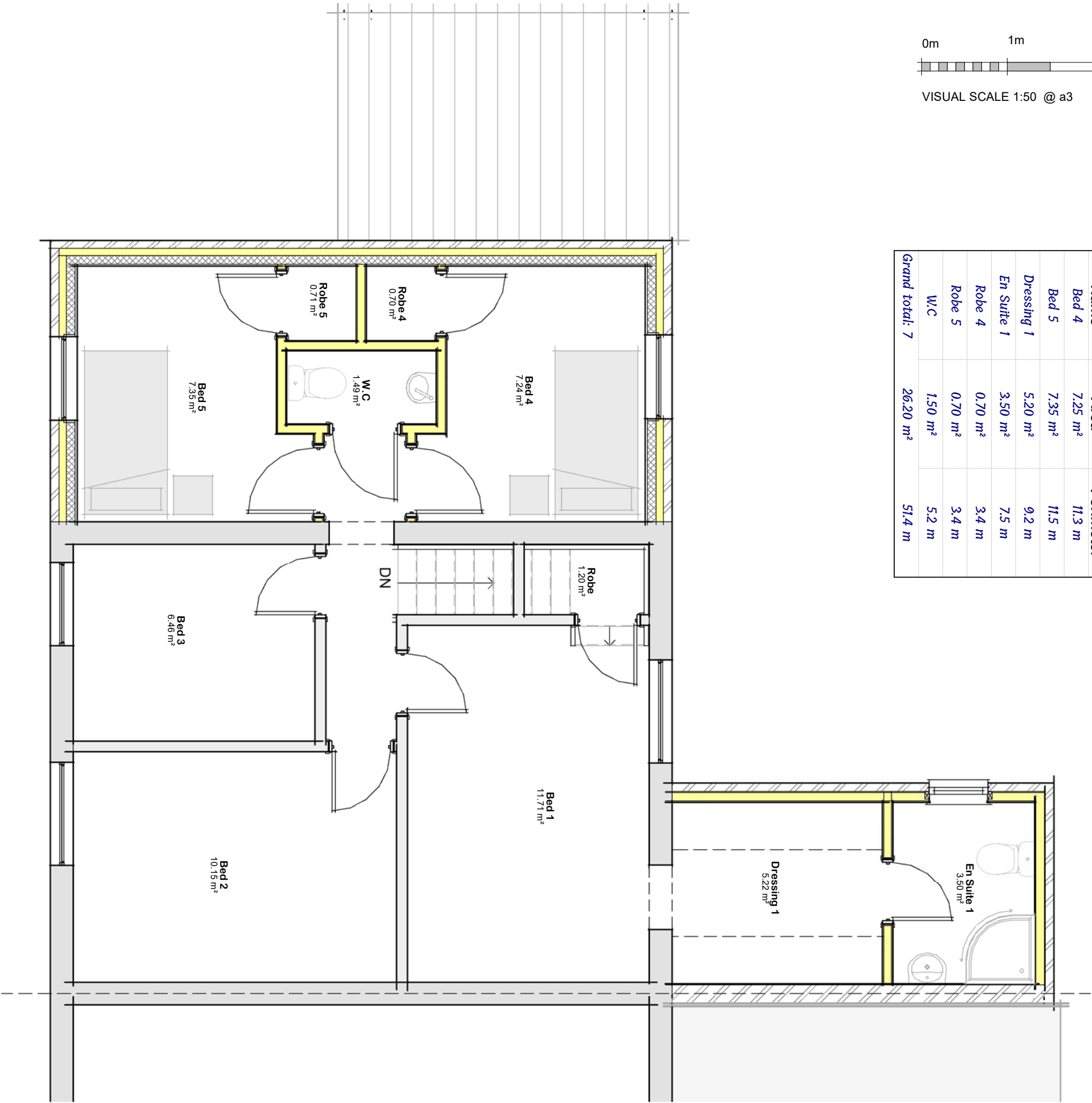
Proposed First Floor Layout
