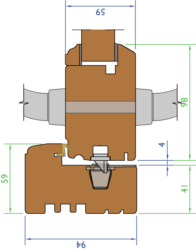
Stable Door Handle L-L - (Scale 1:2)
