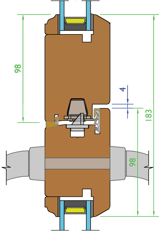
French Door Meeting Thumb Bolt Option - (Scale 1:2)
