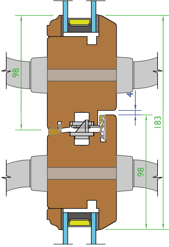
French Door Meeting Concealed Lock Option - (Scale 1:2)
