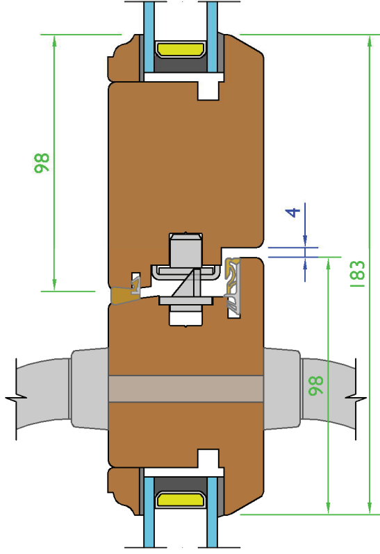
French Door Meeting - (Scale 1:2)
