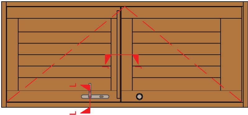
Stable Door - Outside View - (Scale 1:20)
