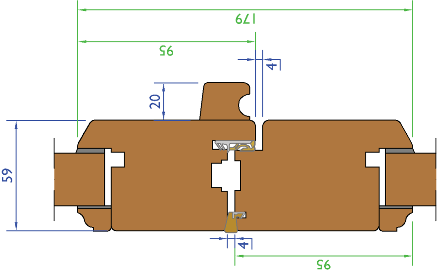
Stable Door Meeting J-J - (Scale 1:2)
