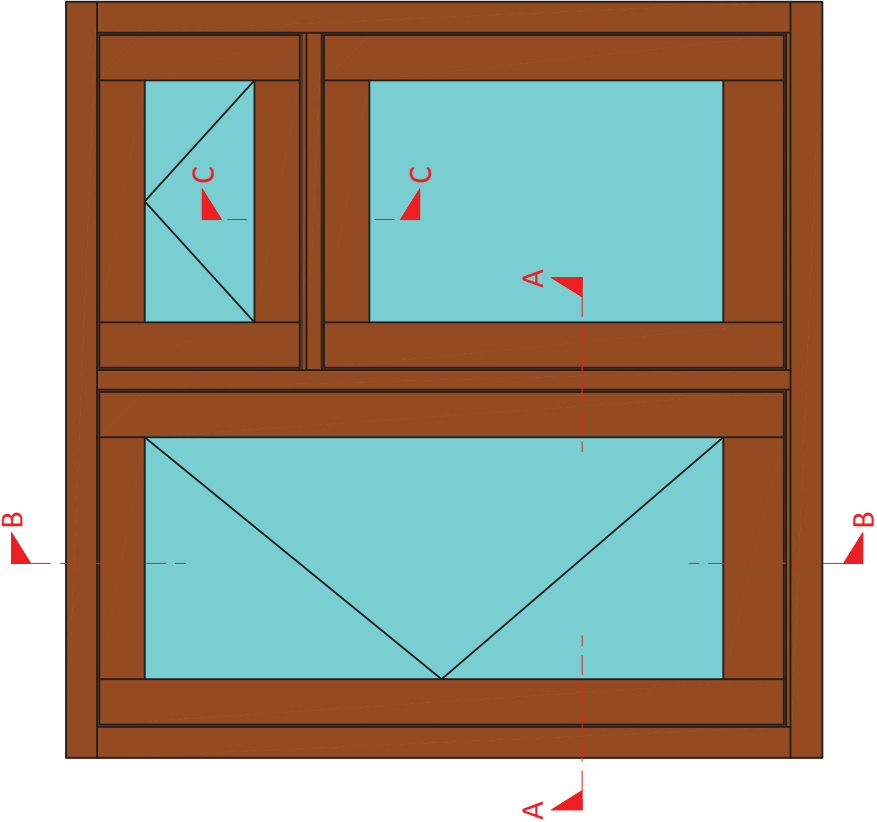
Elevation 1 - Outside View
