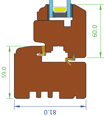
Section A-A - Jamb and mullion
