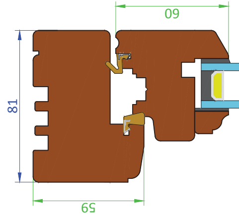
Section B-B - Head and cill
