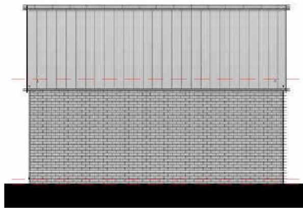
Elevation 03 - Rear 1 : 100
