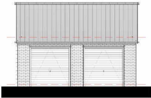
Elevation 01 - Front 1 : 100
