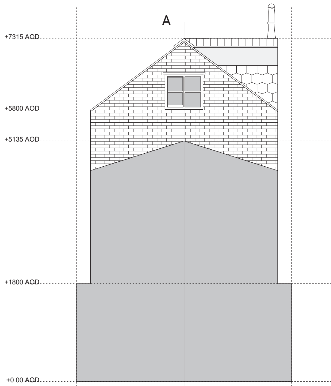
EXISTING EAST ELEVATION
