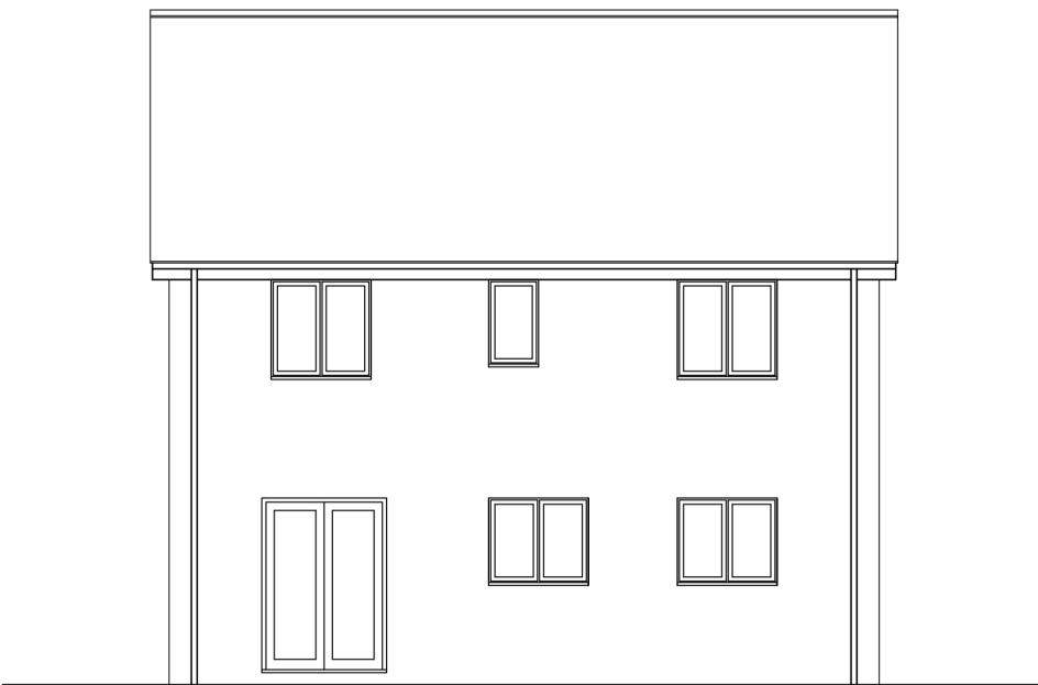
Rear Elevation
