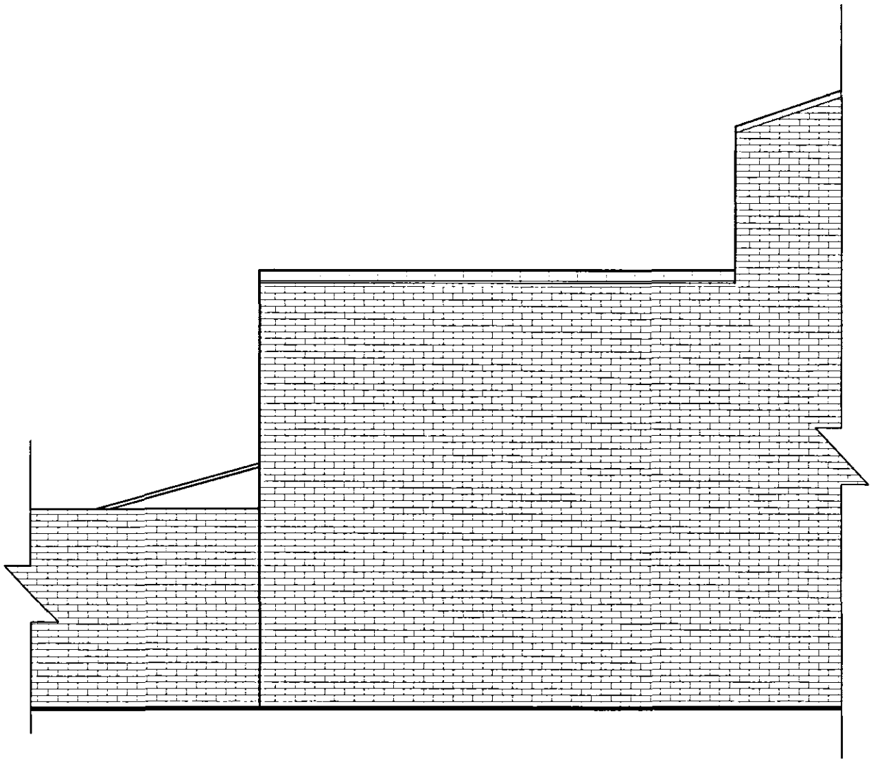
① EXISTING WORKSHOP WING WEST ELEVATION
