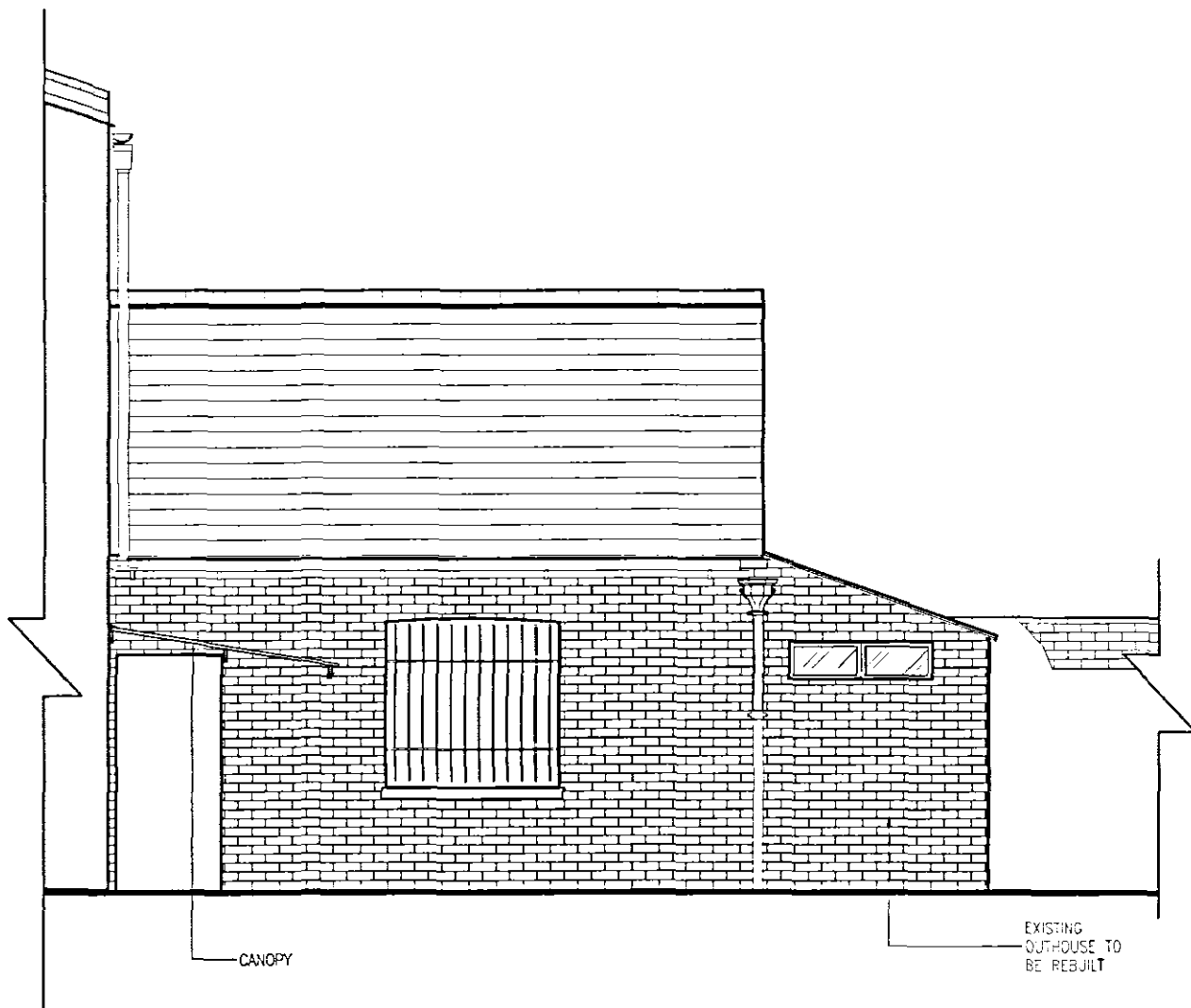
(E) EXISTING WORKSHOP WING EAST ELEVATION
