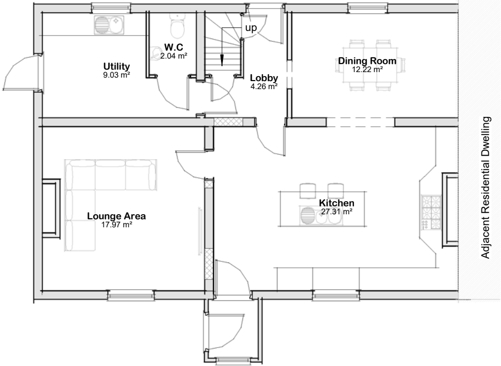
Plan 01 - Ground 1 : 100
