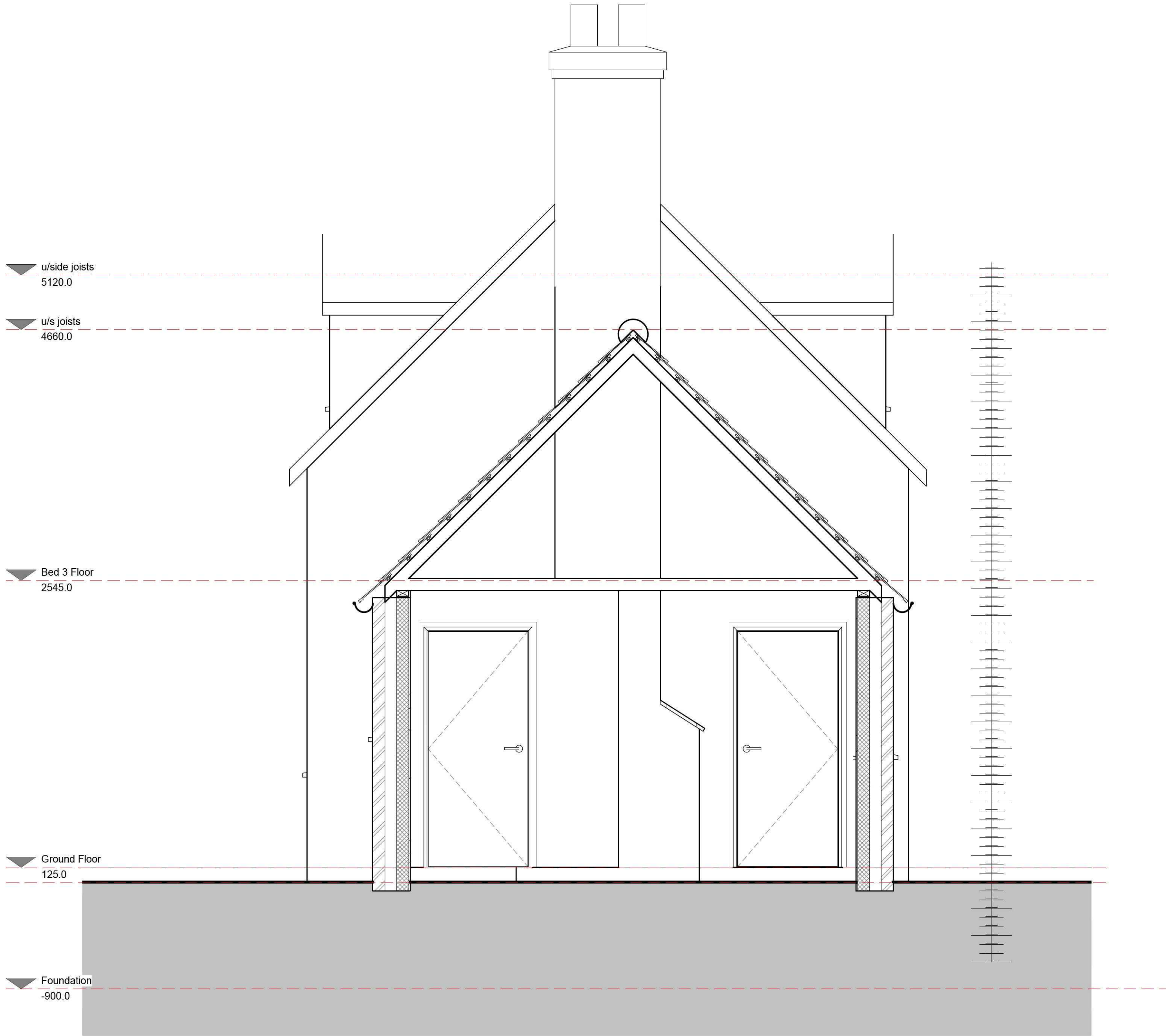
1 Proposed Section 1 : 25
