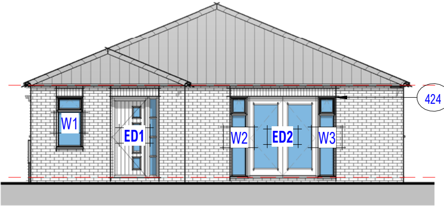
Elevation 01 - Front I : 100
