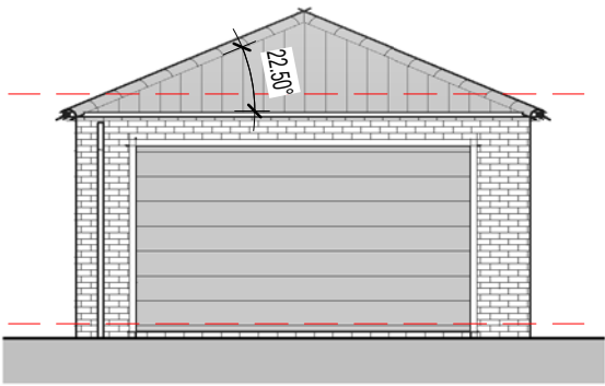
Elevation 01 - Front I : 100
