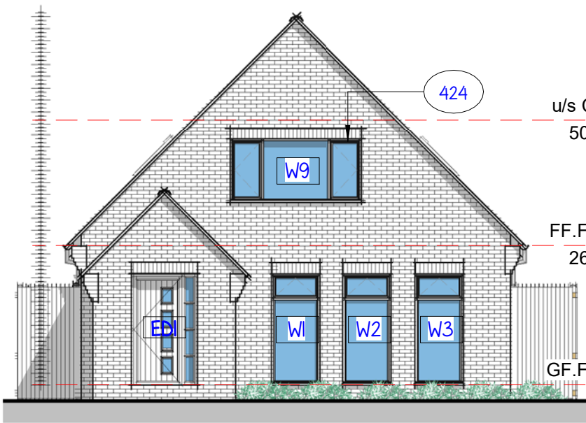
Elevation 01 - Front 1 : 100
