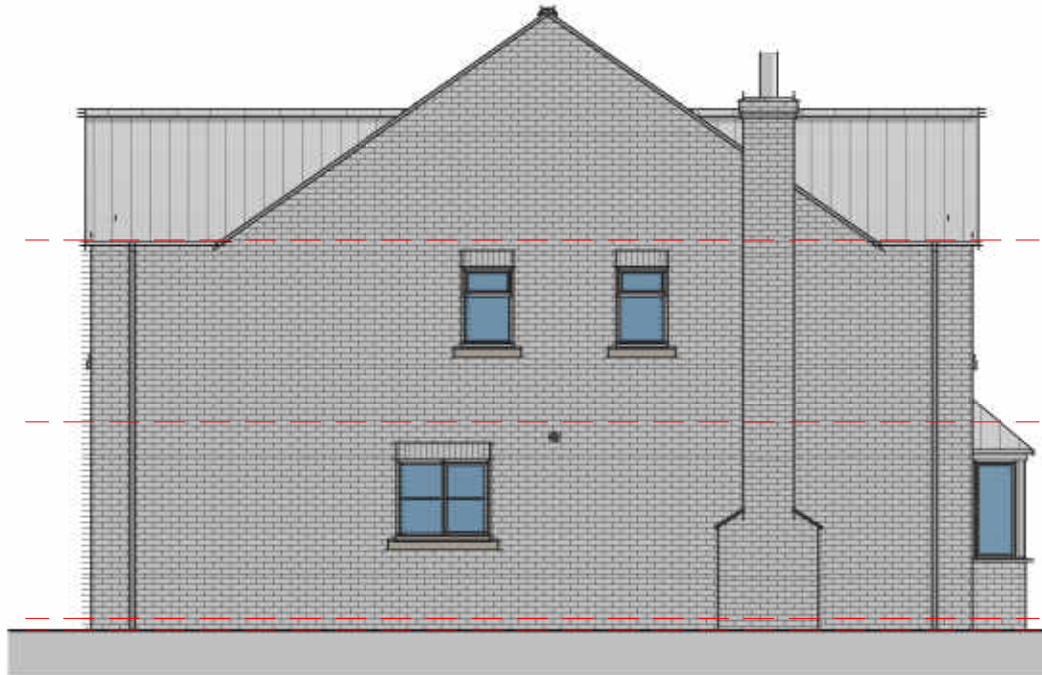
Elevation 04 - Left
