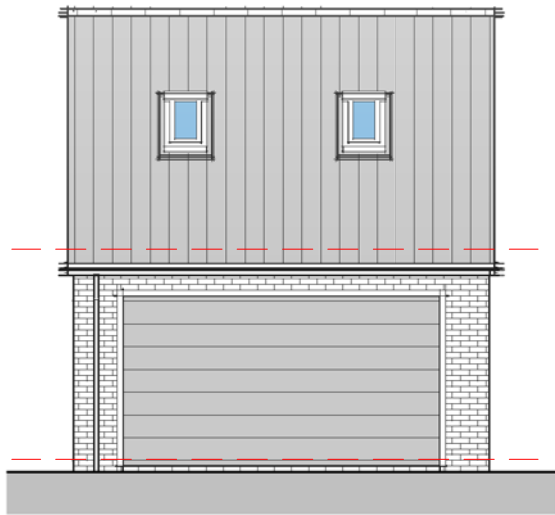
Elevation 01 - Front 1 : 100
