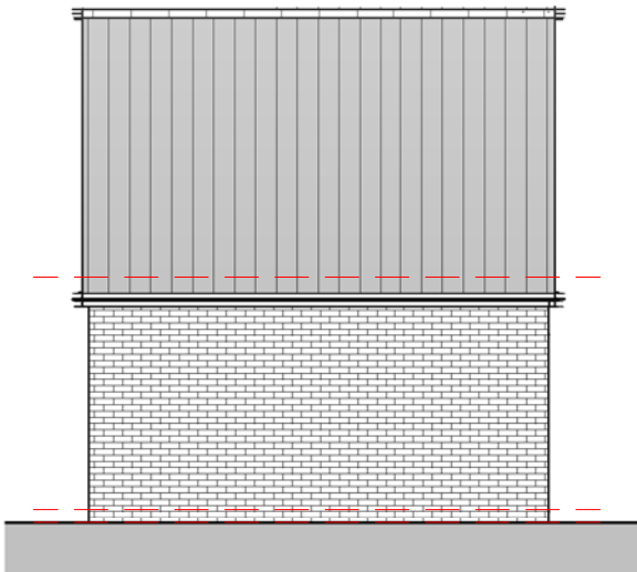
Elevation 03 - Rear 1 : 100
