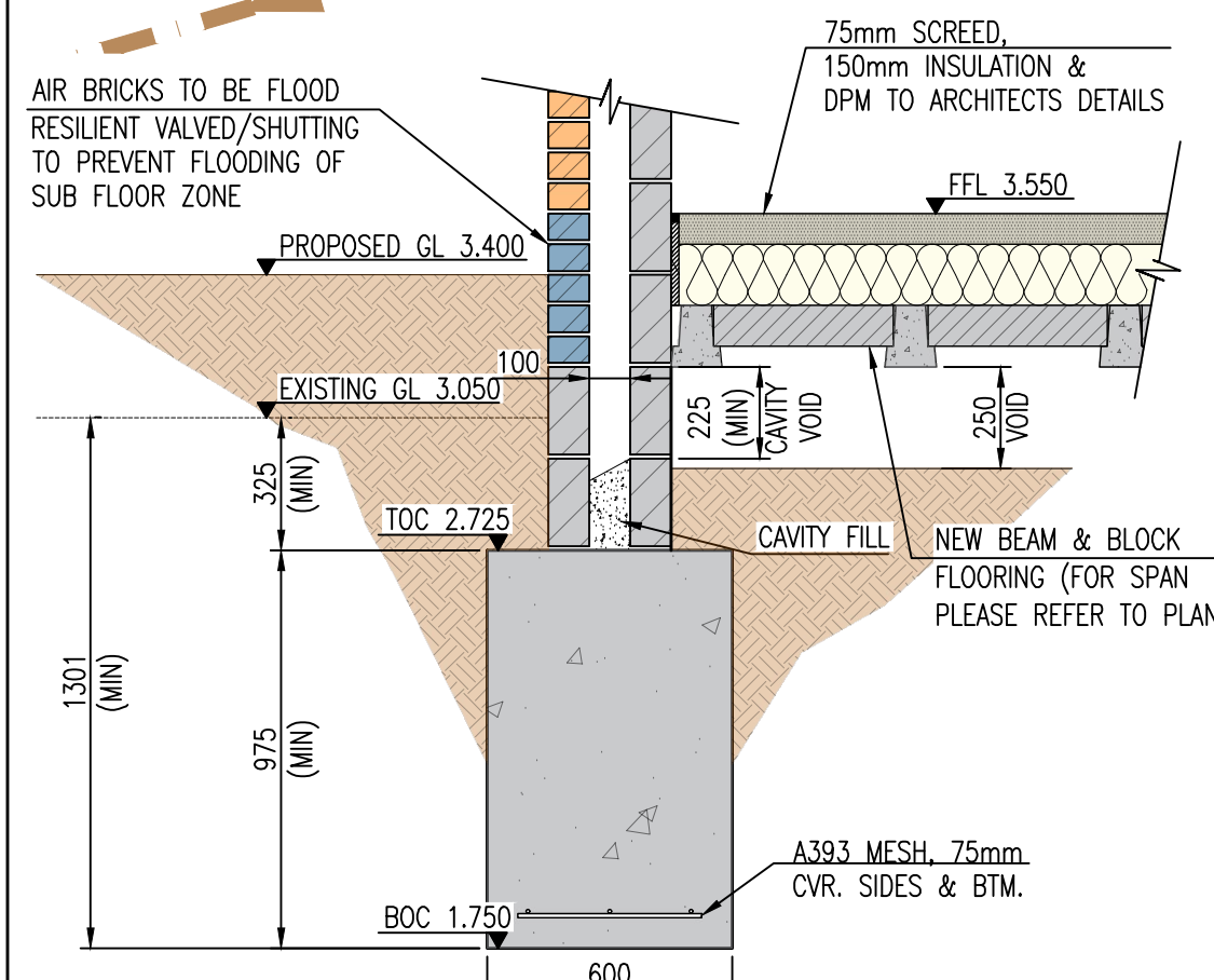
SECTION THROUGH A-A EXTERNAL PERIMETER WALL SCALE 1:20
