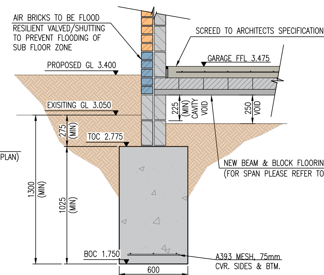
SECTION THROUGH G-G GARAGE EXTERNAL PERIMETER WALL SCALE 1:20
