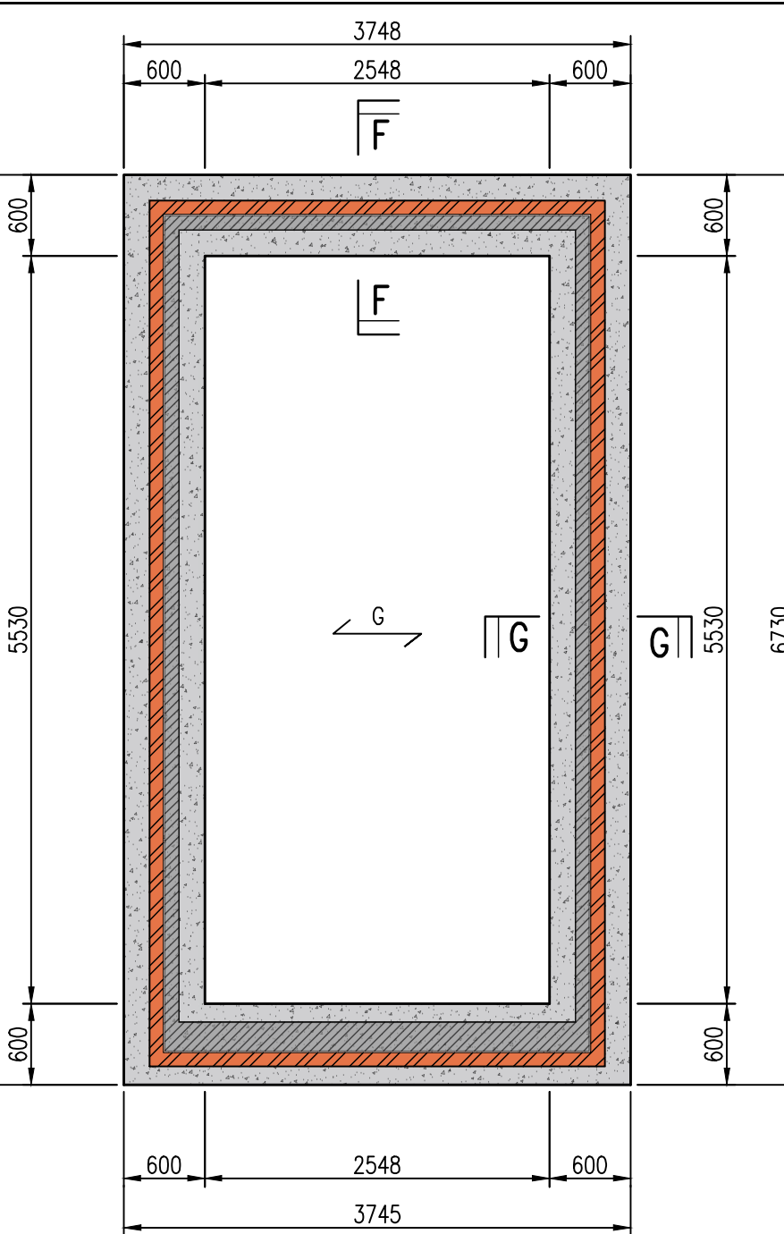
PROPOSED STRIP FOUNDATION ARRANGEMENT – GARAGE OF PLOT 1 SCALE 1:50
