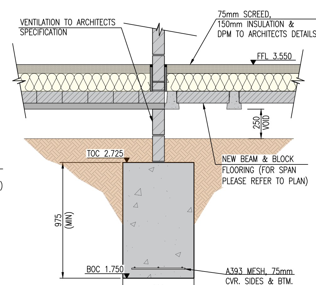
SECTION THROUGH C-C INTERNAL 100mm THK. SLEEPER WALL SCALE 1:20
