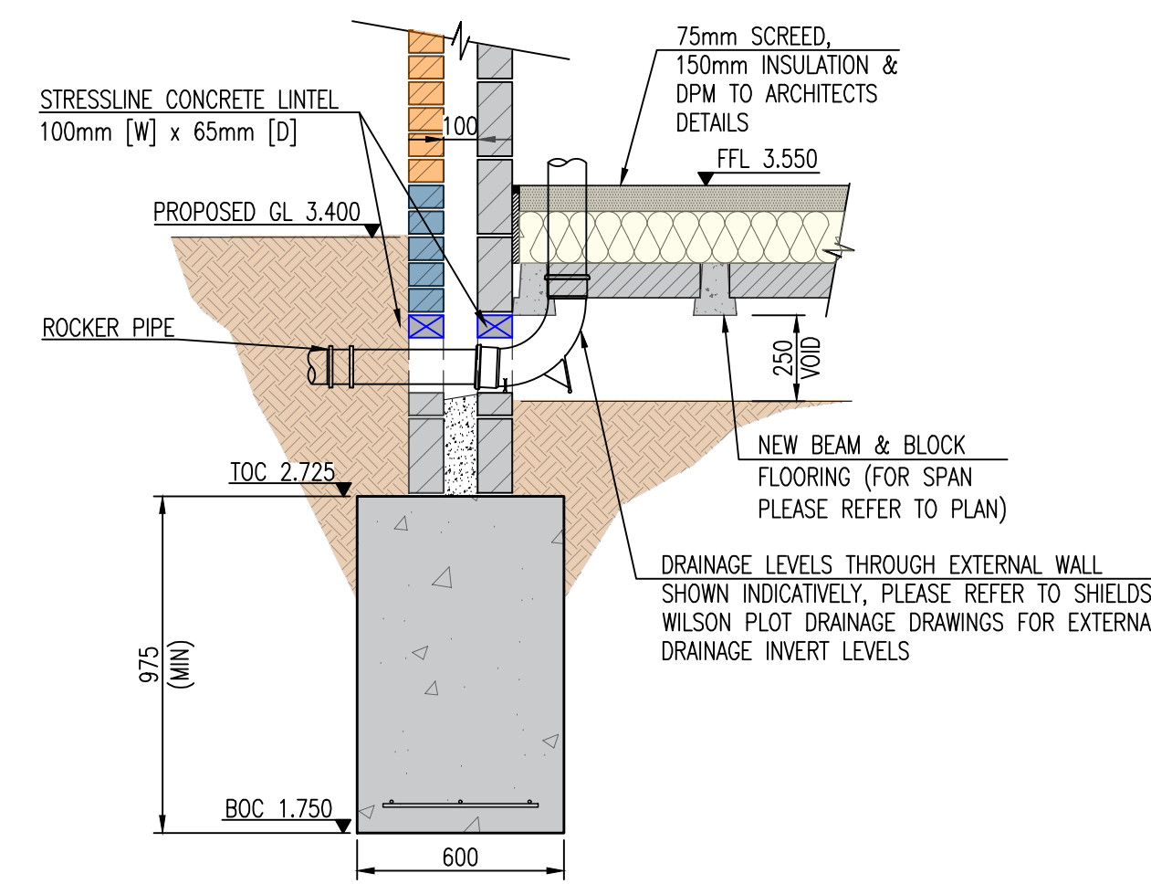
SECTION SHOWING DRAINAGE THROUGH EXTERNAL WALL SCALE 1:20
