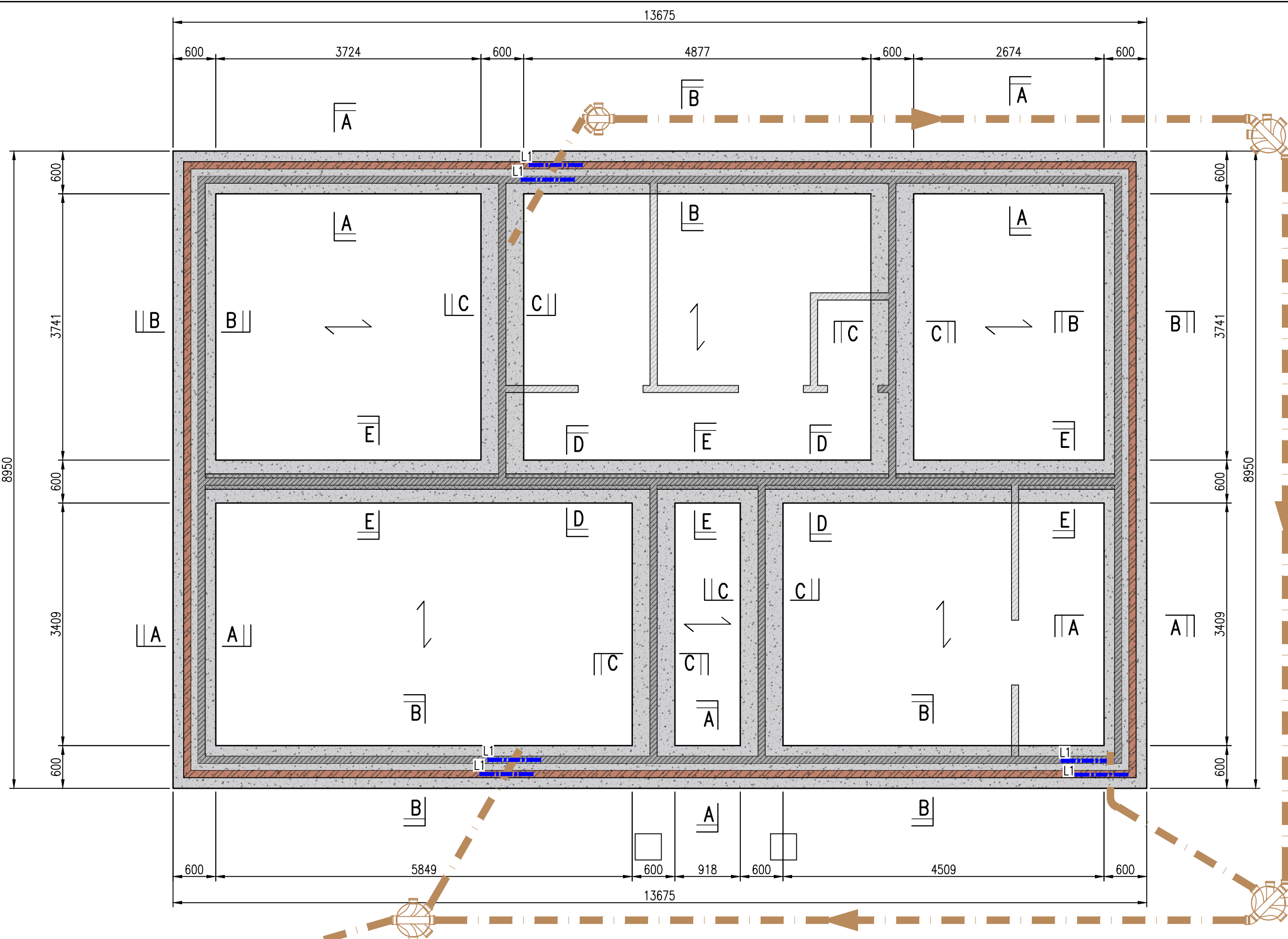
PROPOSED STRIP FOUNDATION ARRANGEMENT – PLOT 1 SCALE 1:50
