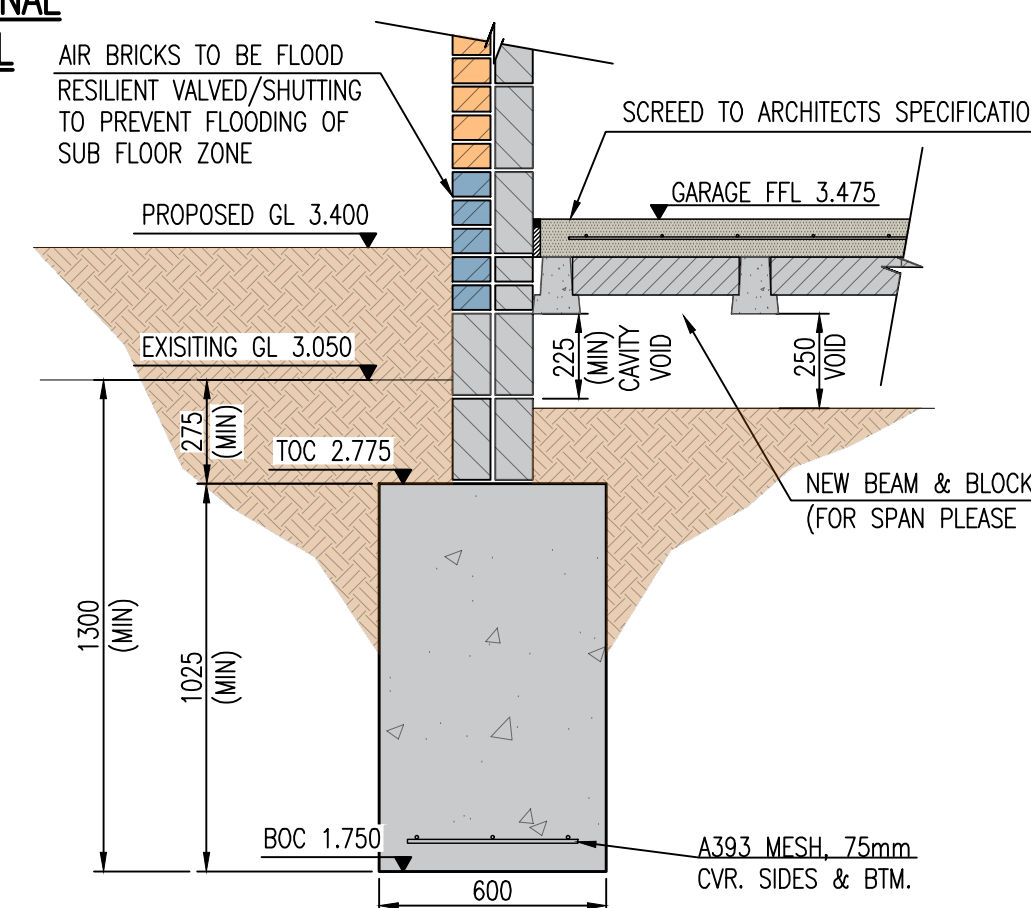
SECTION THROUGH F-F GARAGE EXTERNAL PERIMETER WALL SCALE 1:20
