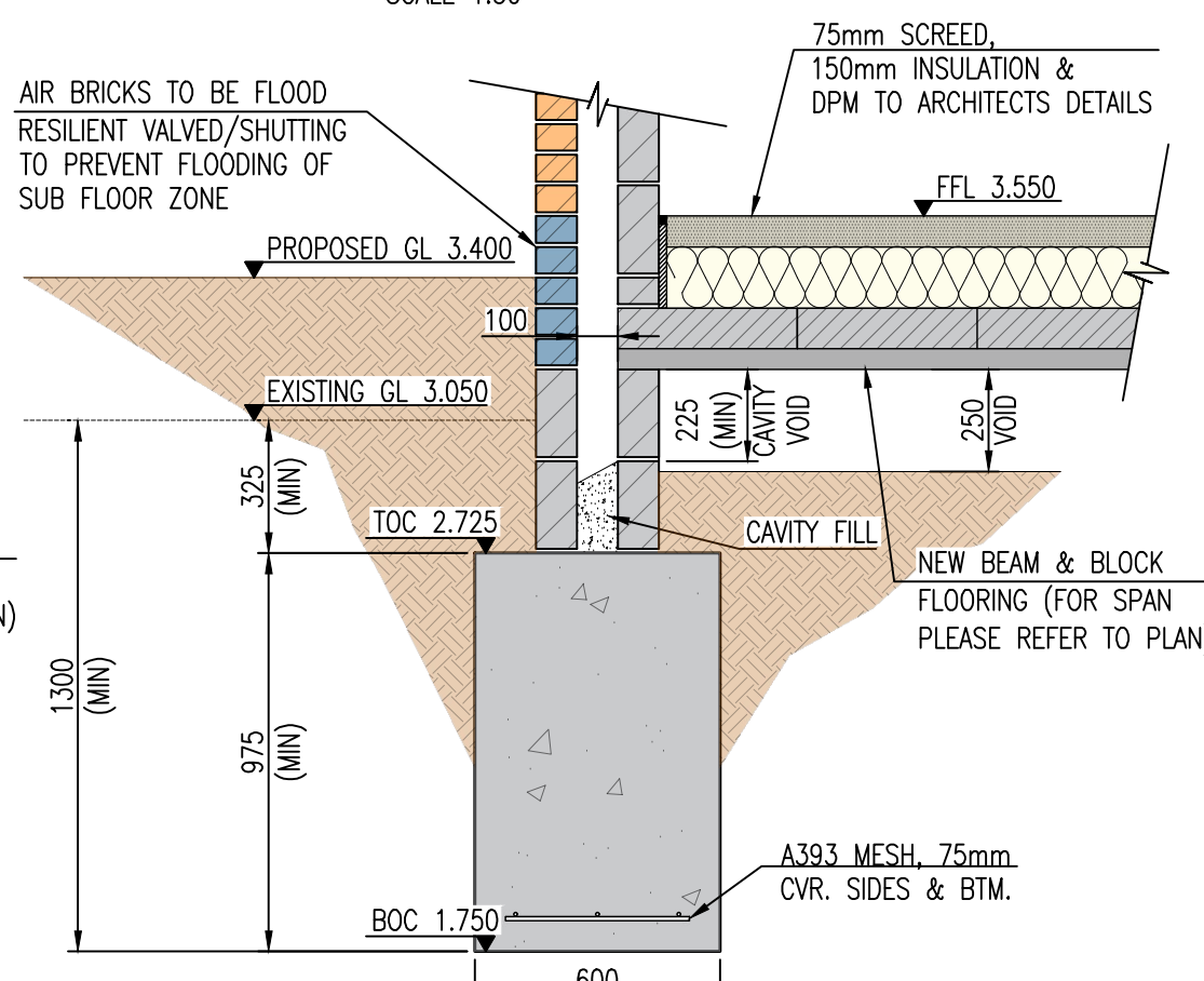
SECTION THROUGH B-B EXTERNAL PERIMETER WALL SCALE 1:20
