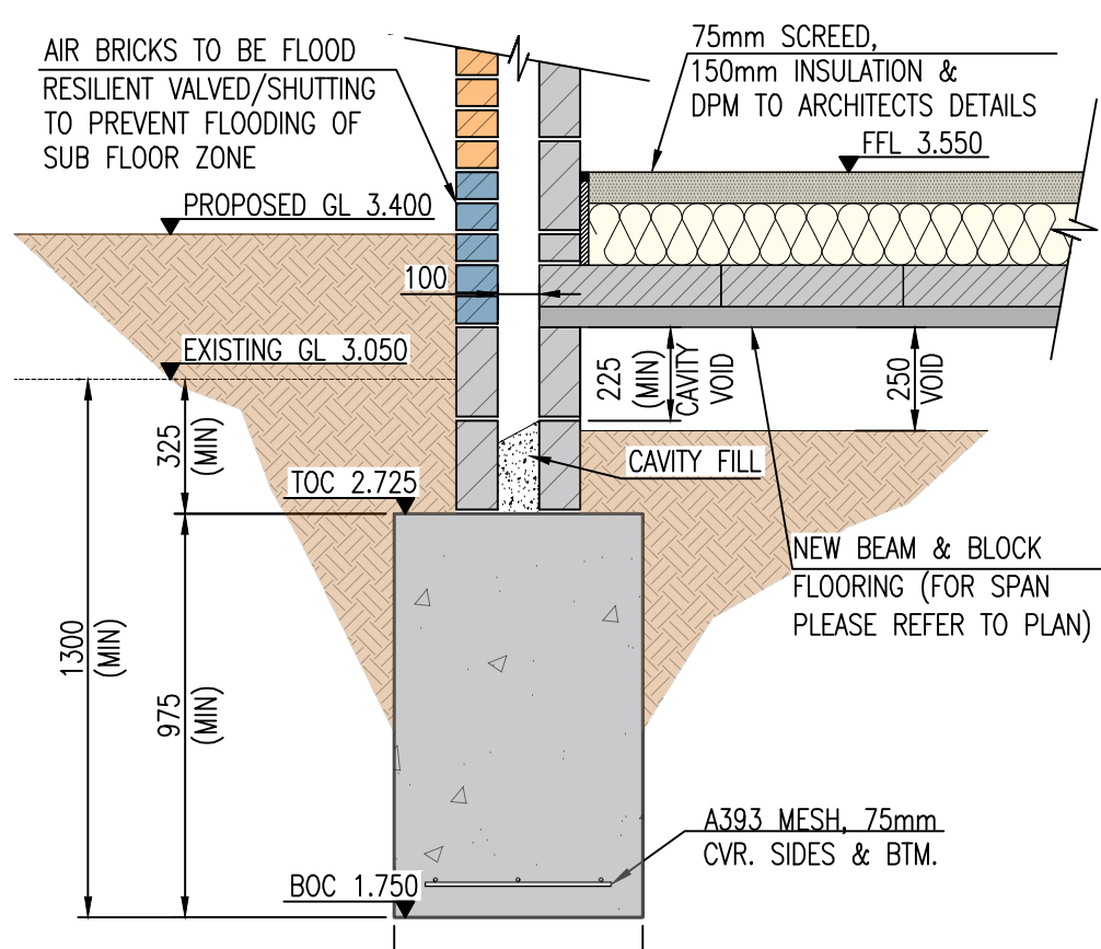
SECTION THROUGH B-B EXTERNAL PERIMETER WALL SCALE 1:20
