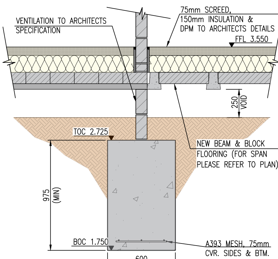
SECTION THROUGH C-C INTERNAL 100mm THK. SLEEPER WALL SCALE 1:20
