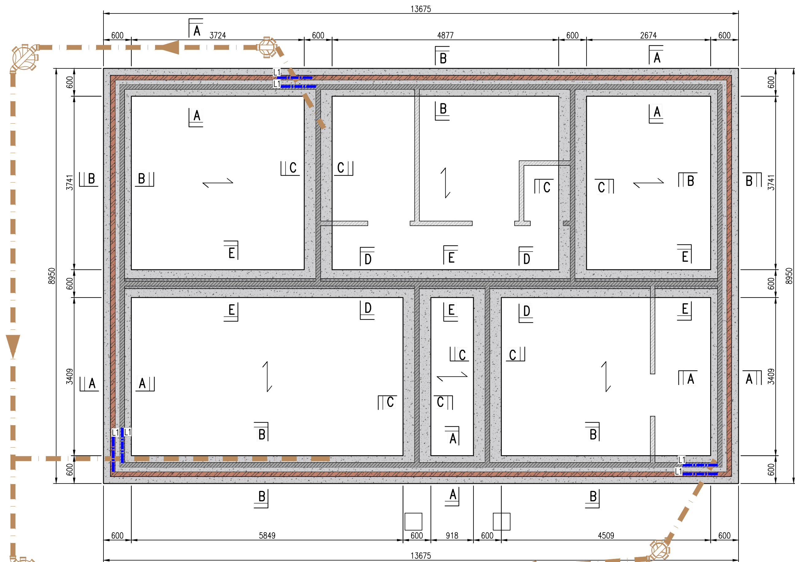
PROPOSED STRIP FOUNDATION ARRANGEMENT – PLOT 6 SCALE 1:50
