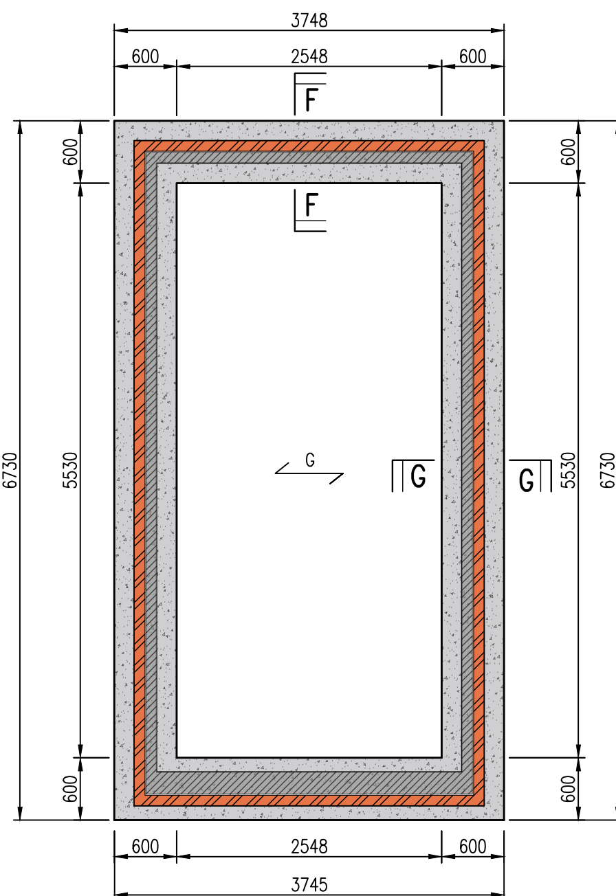
PROPOSED STRIP FOUNDATION ARRANGEMENT – GARAGE OF PLOT 6 SCALE 1:50
