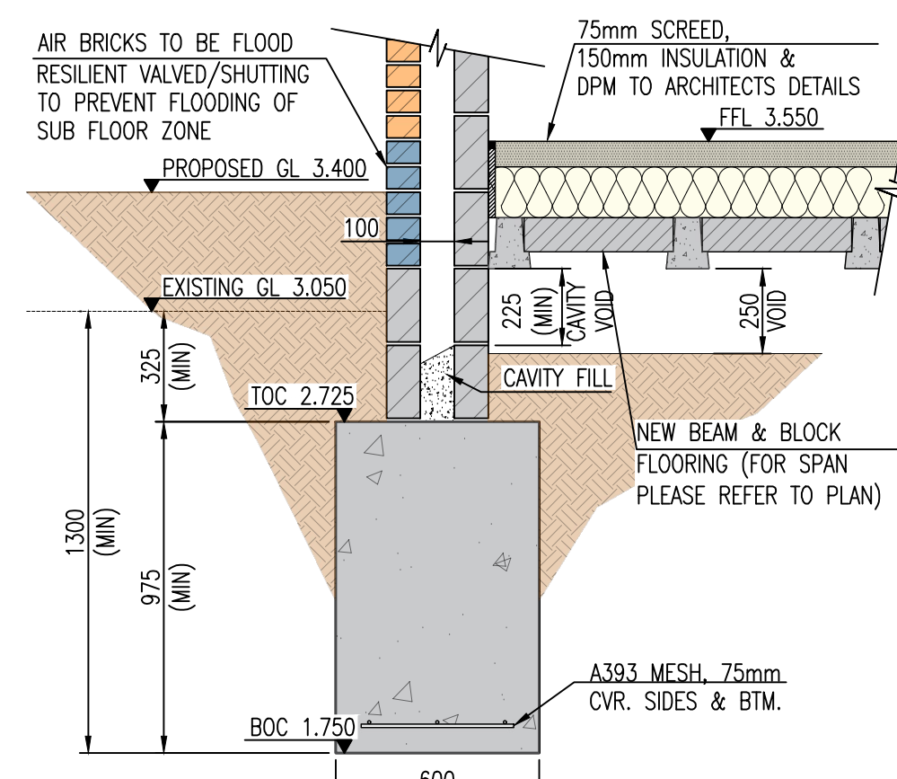
SECTION THROUGH A-A EXTERNAL PERIMETER WALL SCALE 1:20
