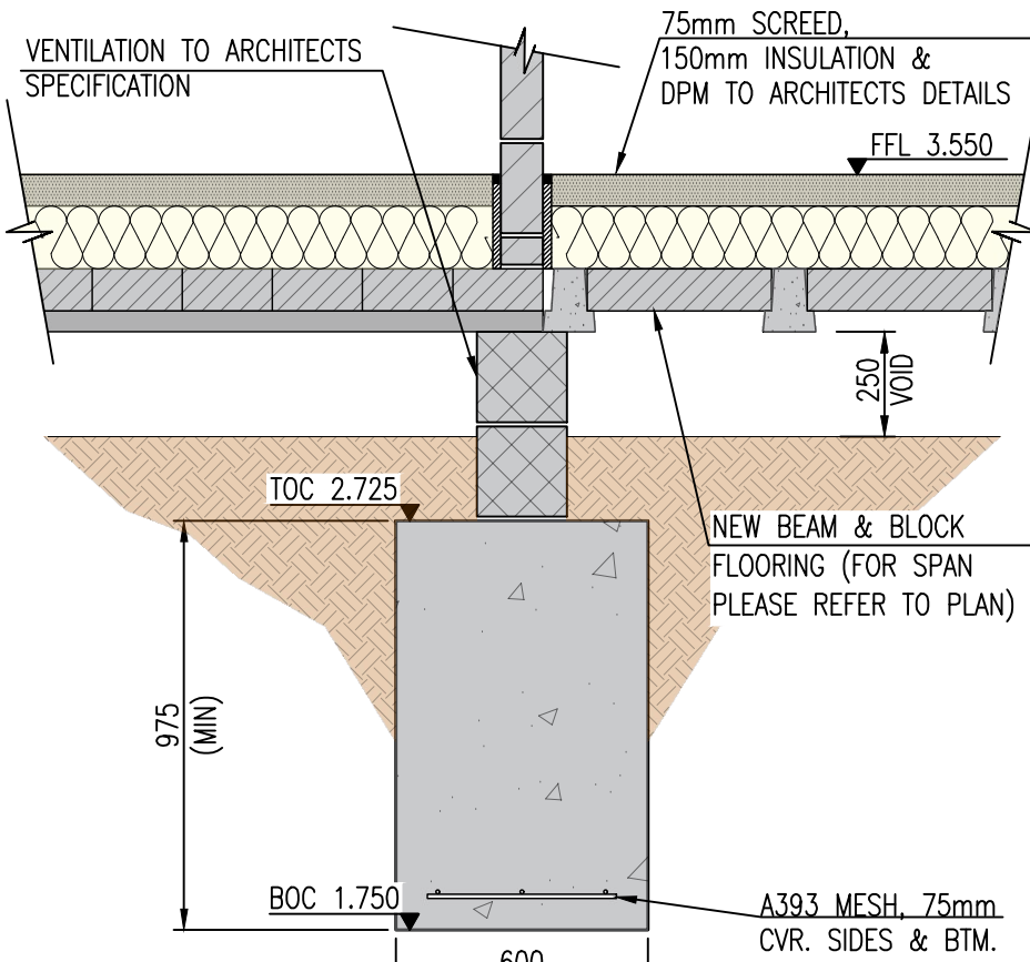
SECTION THROUGH E-E INTERNAL 215mm THK. SLEEPER WALL SCALE 1:20
