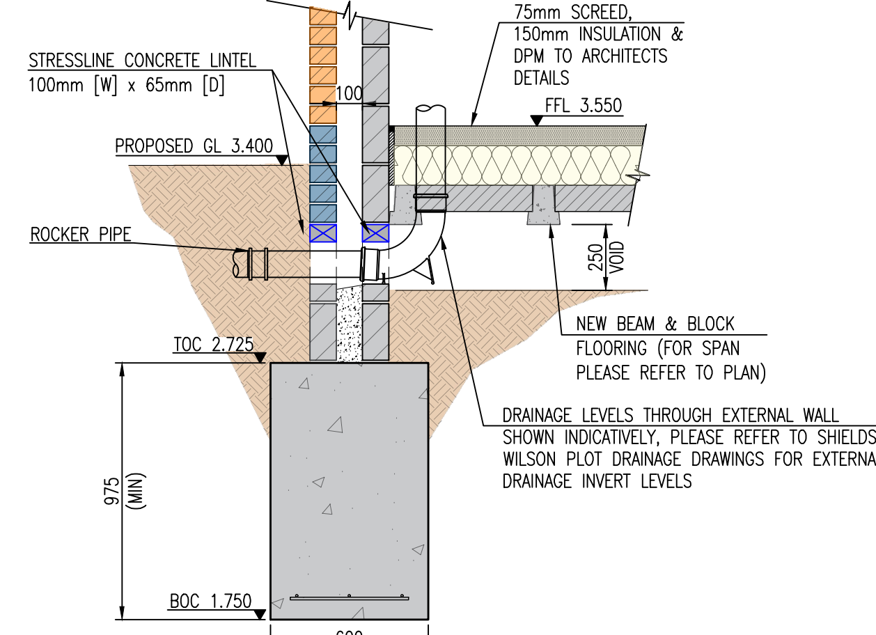
SECTION SHOWING DRAINAGE THROUGH EXTERNAL WALL SCALE 1:20
