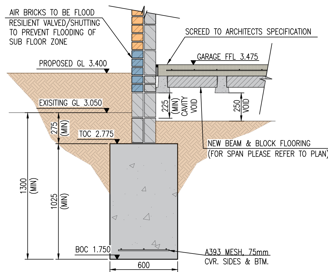
SECTION THROUGH F-F GARAGE EXTERNAL PERIMETER WALL SCALE 1:20
