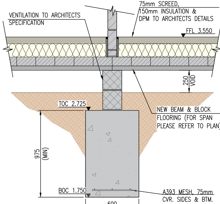
SECTION THROUGH D-D INTERNAL 215mm THK. SLEEPER WALL SCALE 1:20
