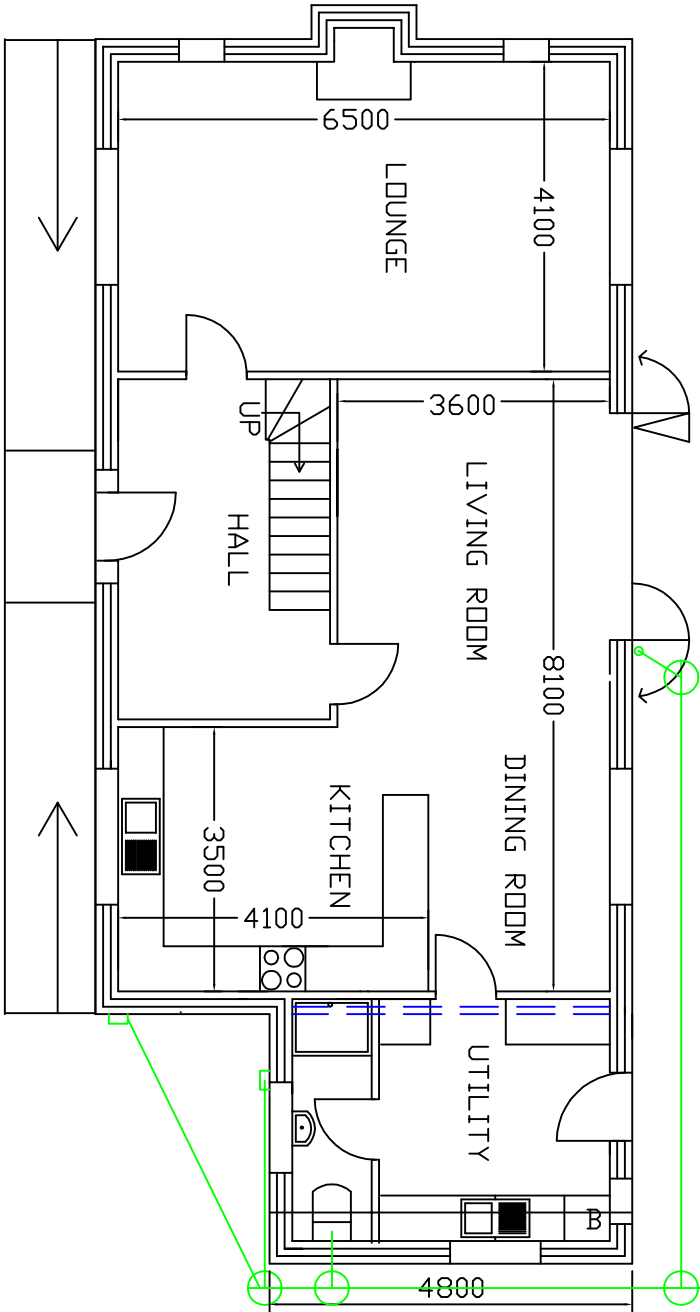
PROPOSED GROUND FLOOR LAYOUT 1:100
