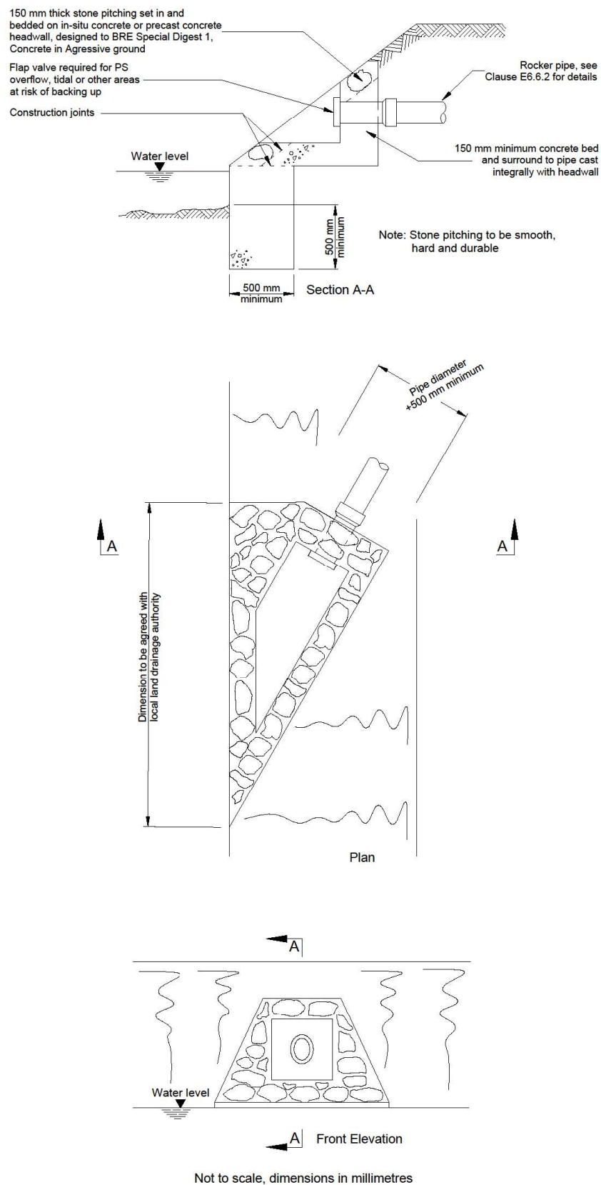
Figure C 2 Typical detail of angled outfall to watercourse Suitable for outfall pipes of less than 350 mm
