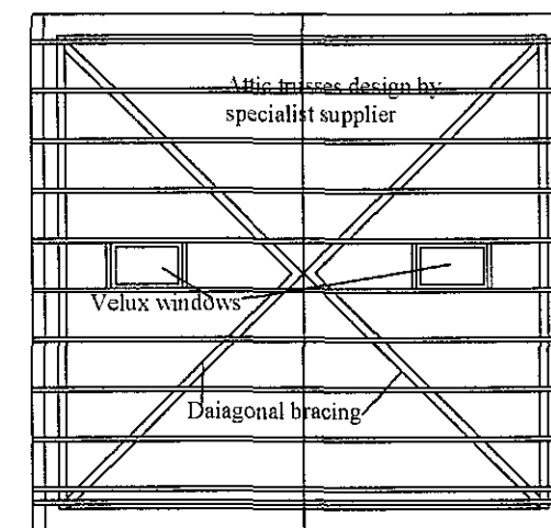
ROOF STRUCTURE
