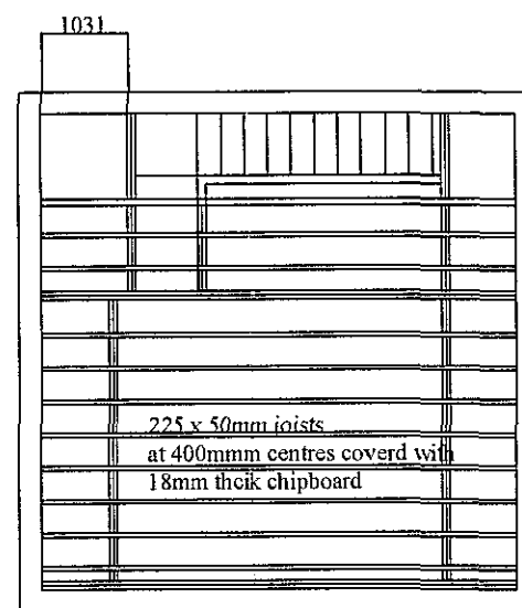
FIRST FLOOR STRUCTURE
