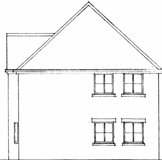
south elevation
