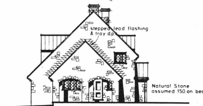
SIDE ELEVATION
