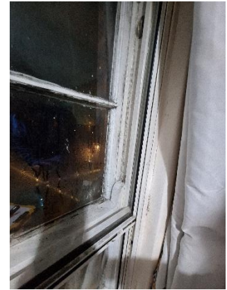
Existing timber windows in a deteriorating but repairable condition. Secondary glazing internally.
