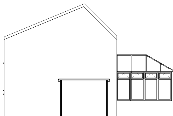
4 West Elevation - (Existing) 1 : 100
