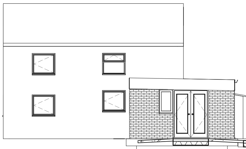
1 North Elevation - (Proposed) 1 : 100
