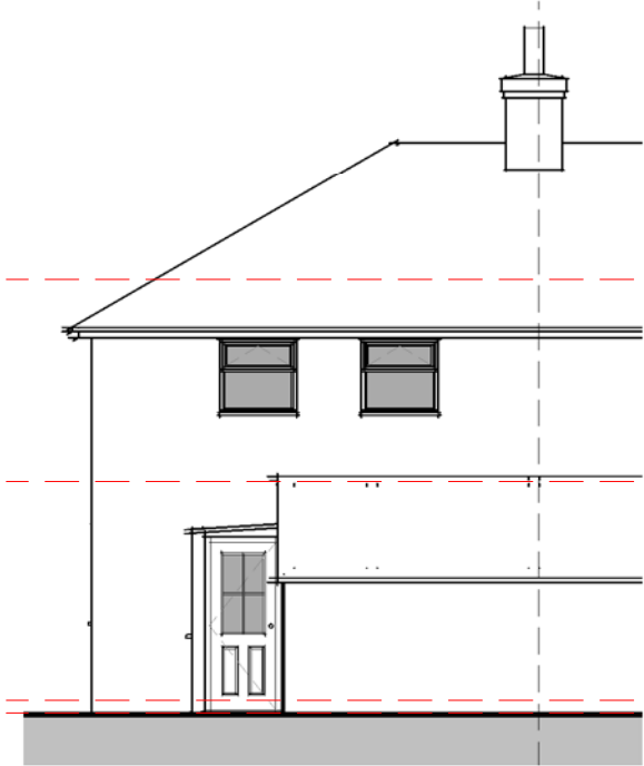
Elevation 03 - Rear 1 : 100
