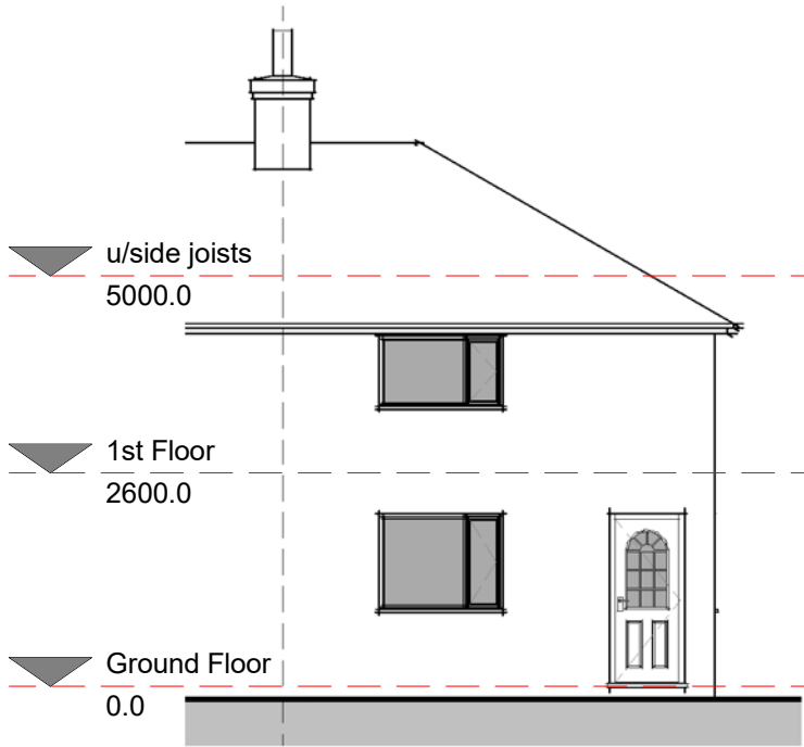
Elevation 01 - Front 1 : 100
