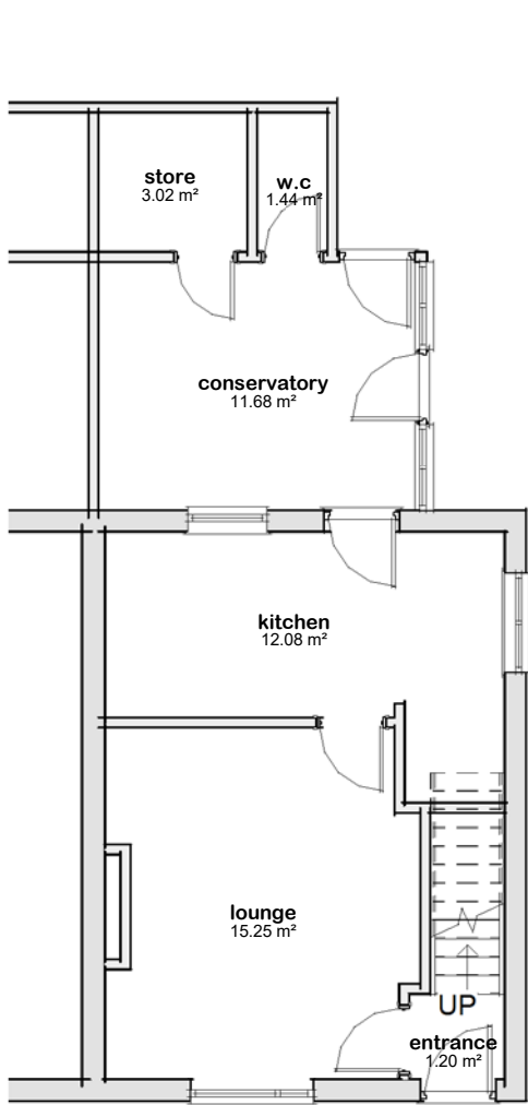
Plan 01 - Ground 1 : 100
