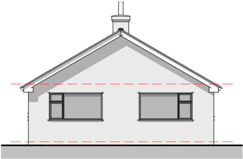
Elevation 01 - Front
