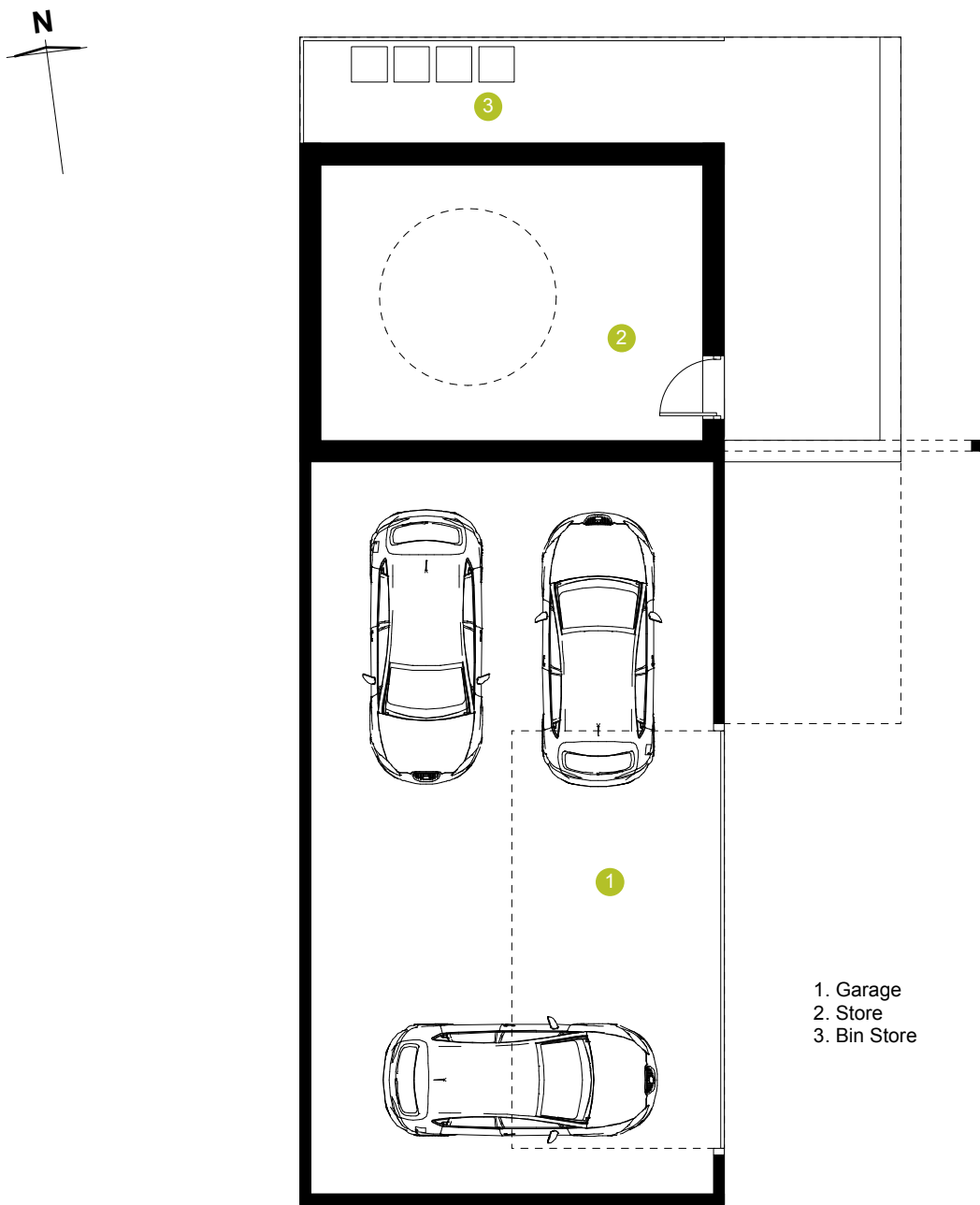
PROPOSED GARAGE FLOOR PLAN 1:100
