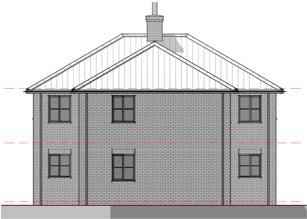
Elevation 03 – Rear 1 : 100
