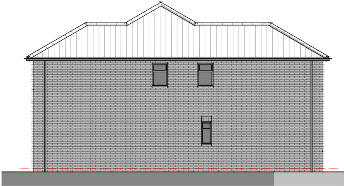
Elevation 04 – Left 1 : 100
