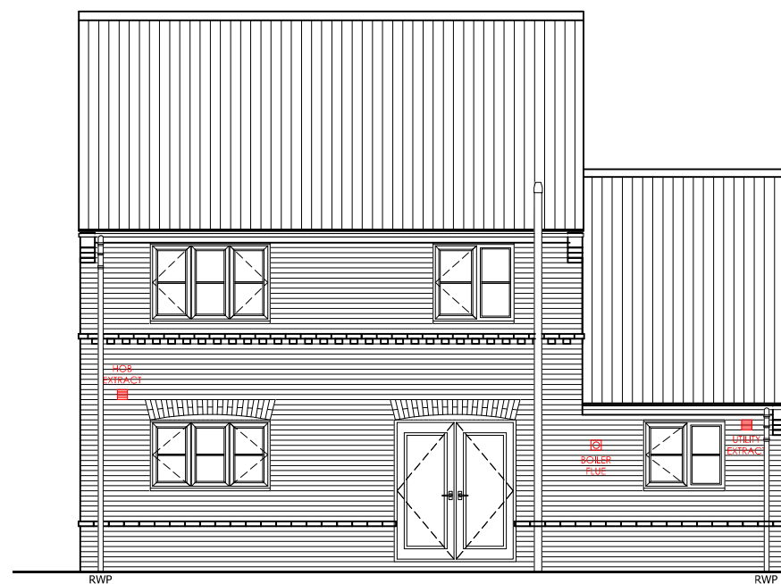
REAR ELEVATION
