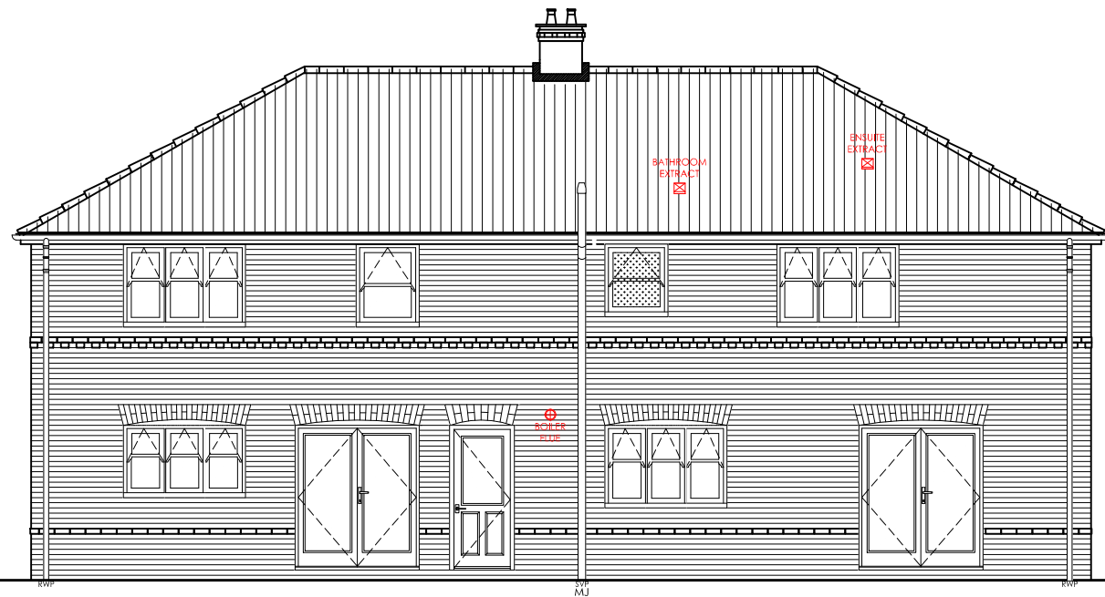
REAR ELEVATION
