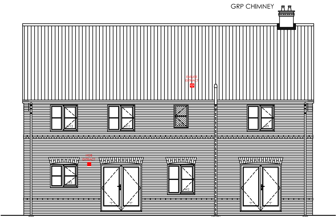
REAR ELEVATION
