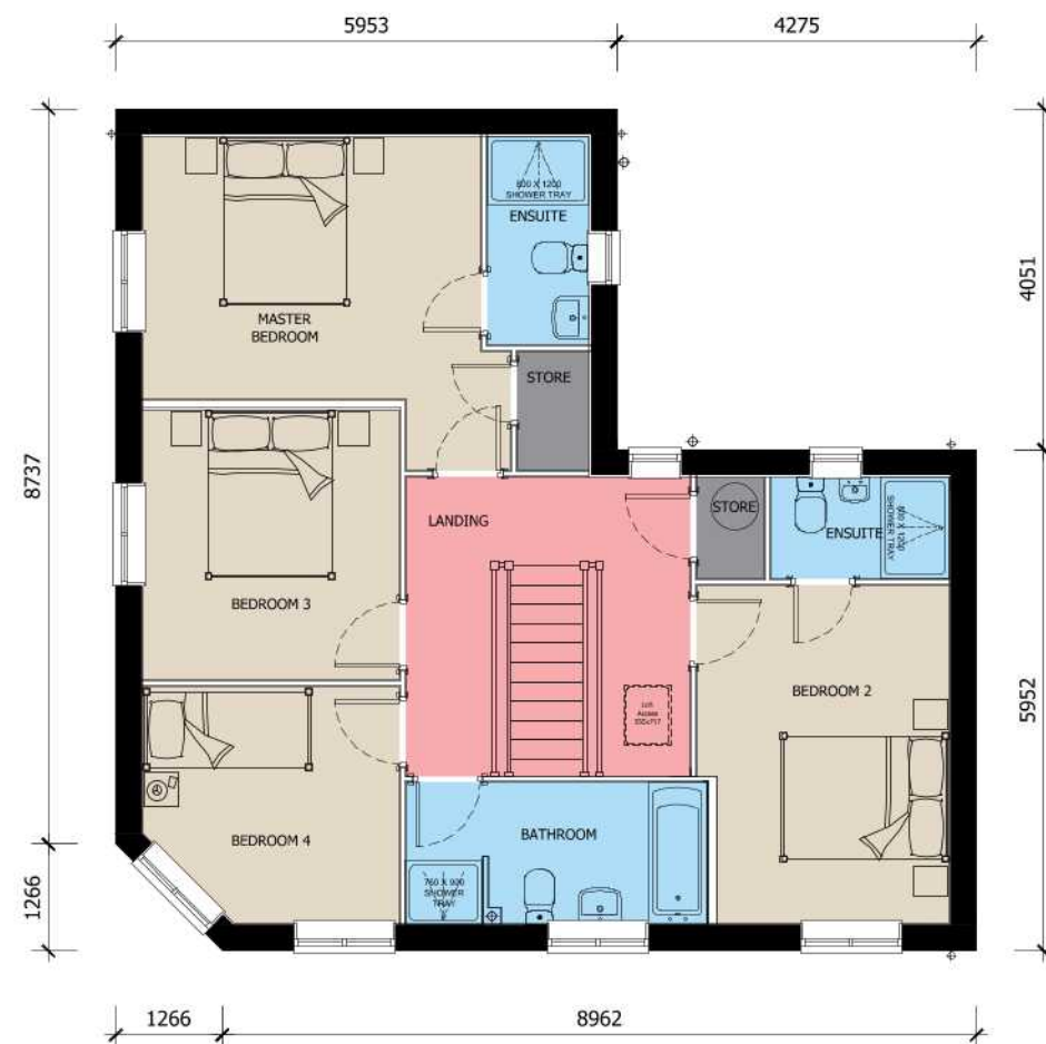
FIRST FLOOR
