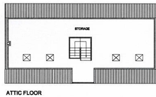
FLOOR PLANS 1:100
