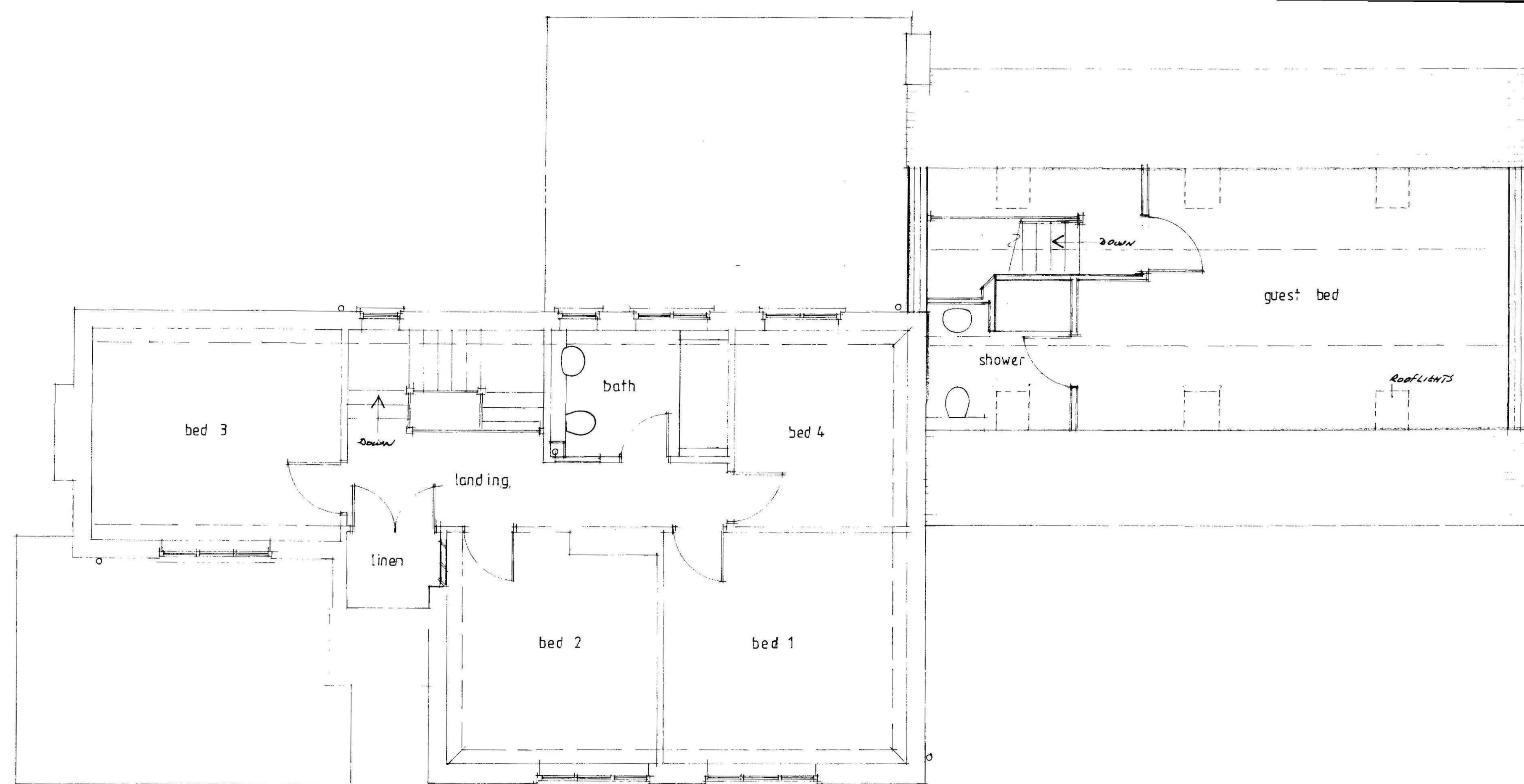
FIRST FLOOR 1:50
