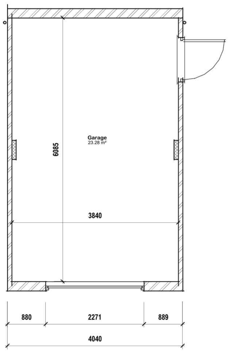
Plan 01 - Ground 1 : 50
