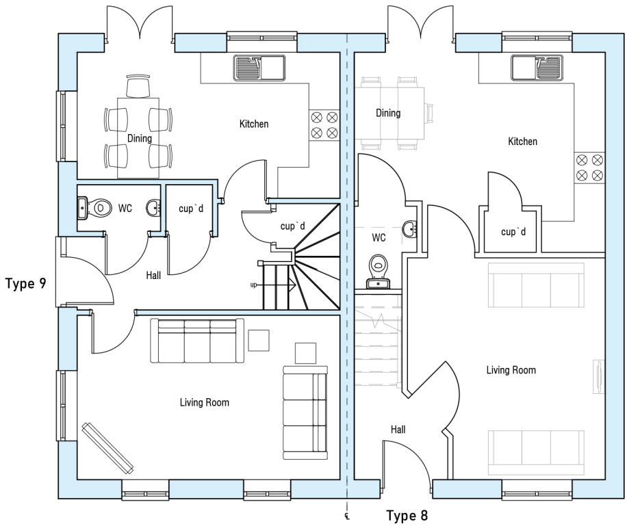
Ground Floor Layout Type 9 & Type 8
