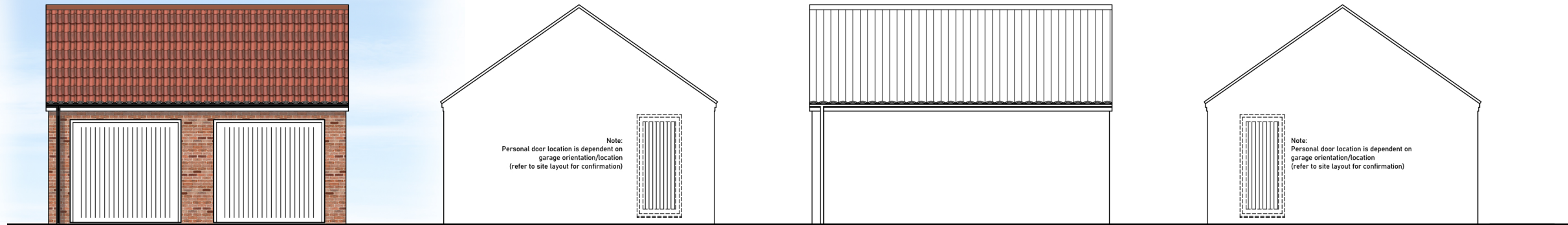
Front Elevation (Double & Twin) Right Side Elevation Rear Elevation Left Side Elevation
