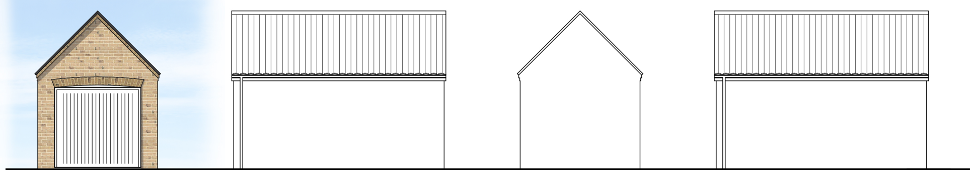
Front Elevation (Single) Right Side Elevation Rear Elevation Left Side Elevation
