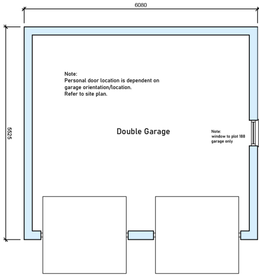
Double Garage Plan
