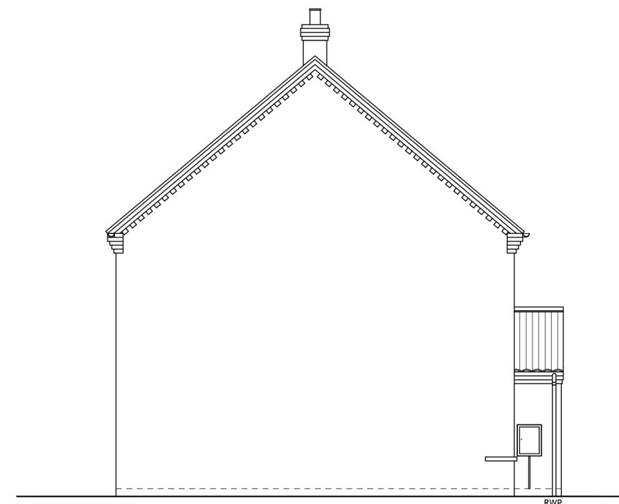
SIDE ELEVATION
