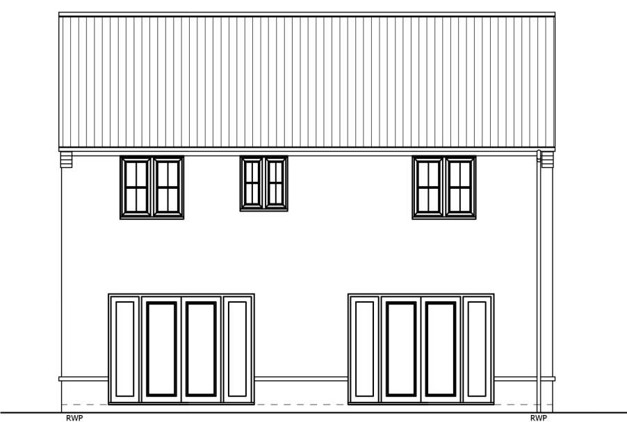
REAR ELEVATION
