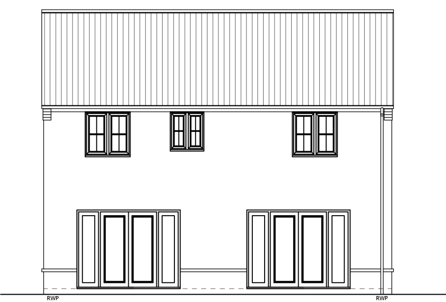
REAR ELEVATION
