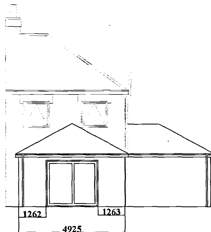
REAR ELEVATION
