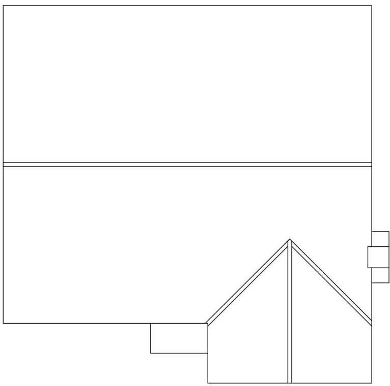
Roof Plan
